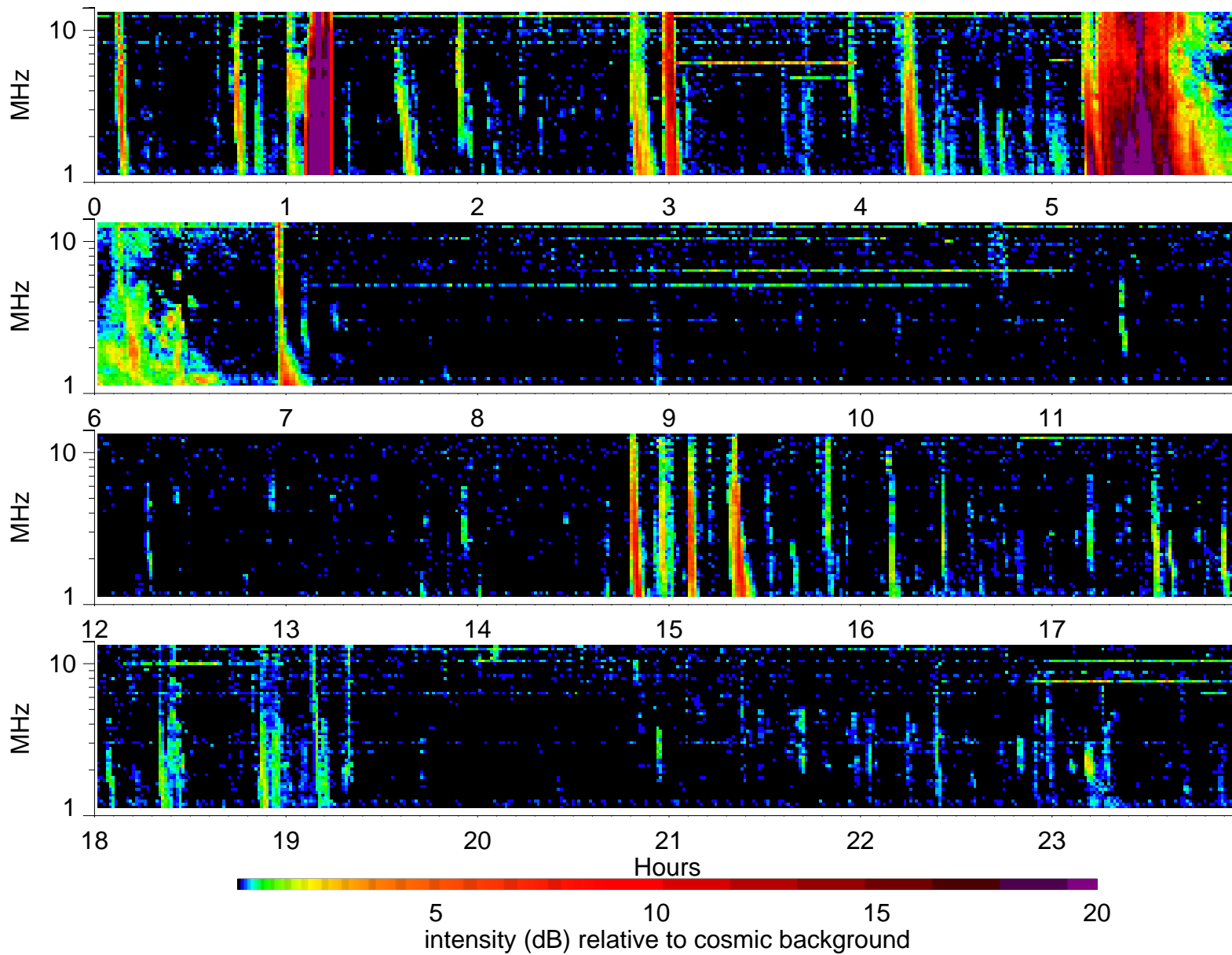
Wind Waves RAD2 receiver: 2001/4/10
