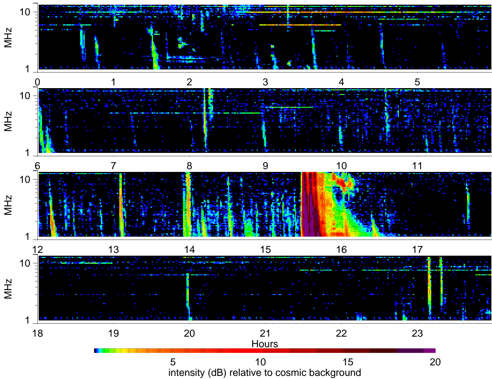
Wind Waves RAD2 receiver: 2001/4/9
