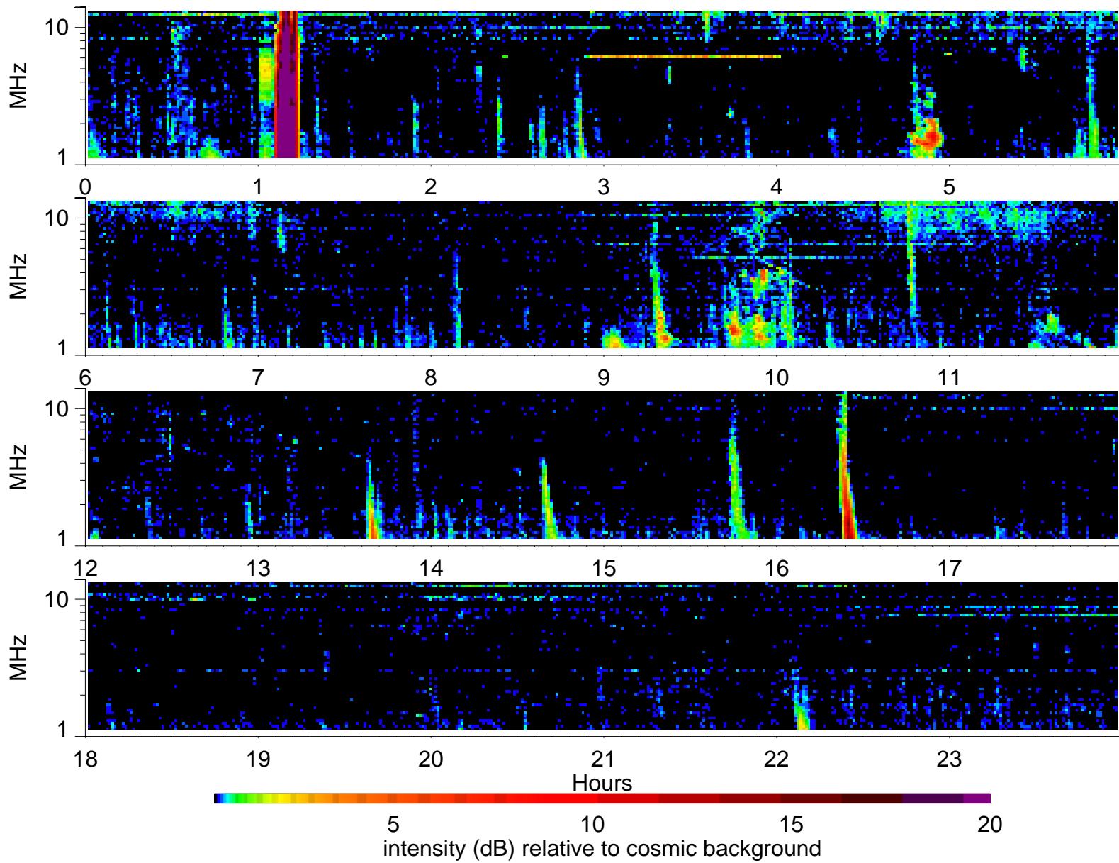
Wind Waves RAD2 receiver: 2001/4/4
