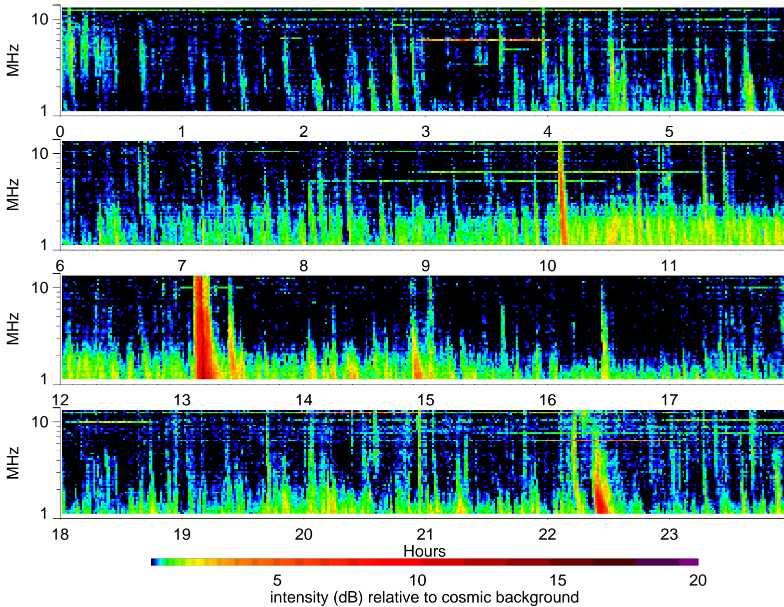
Wind Waves RAD2 receiver: 2001/3/26
