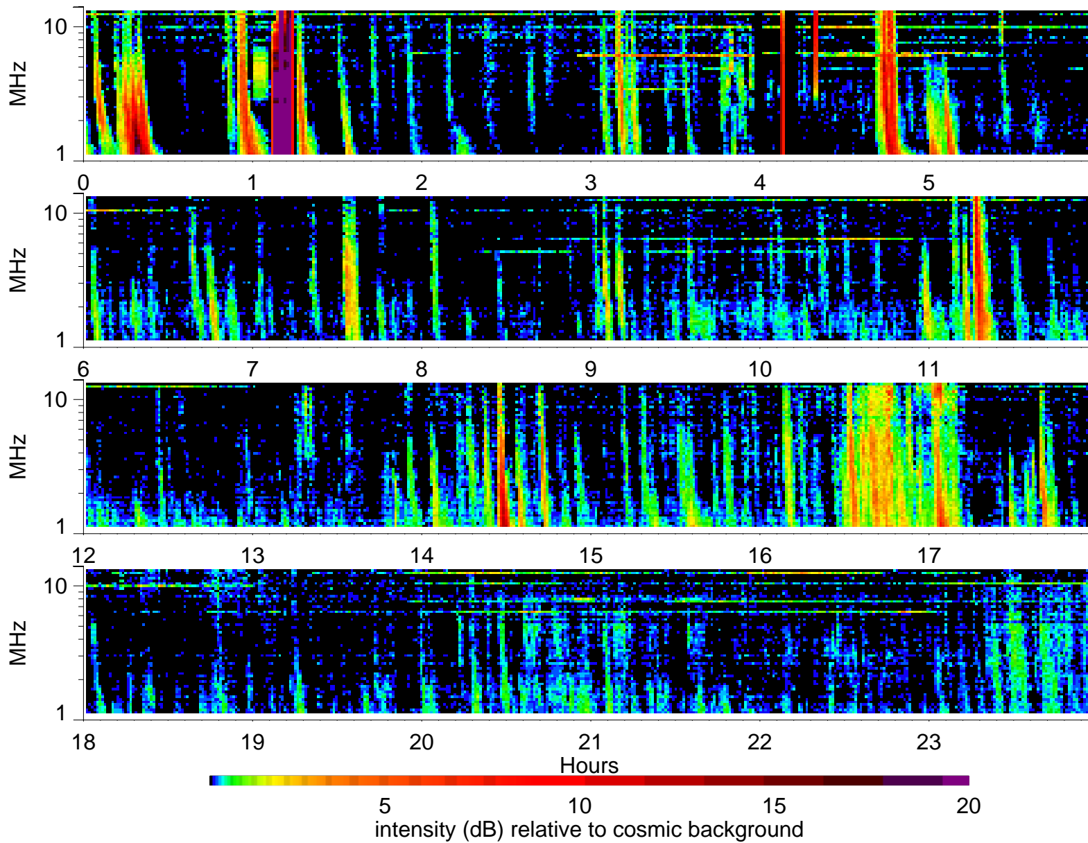
Wind Waves RAD2 receiver: 2001/3/25
