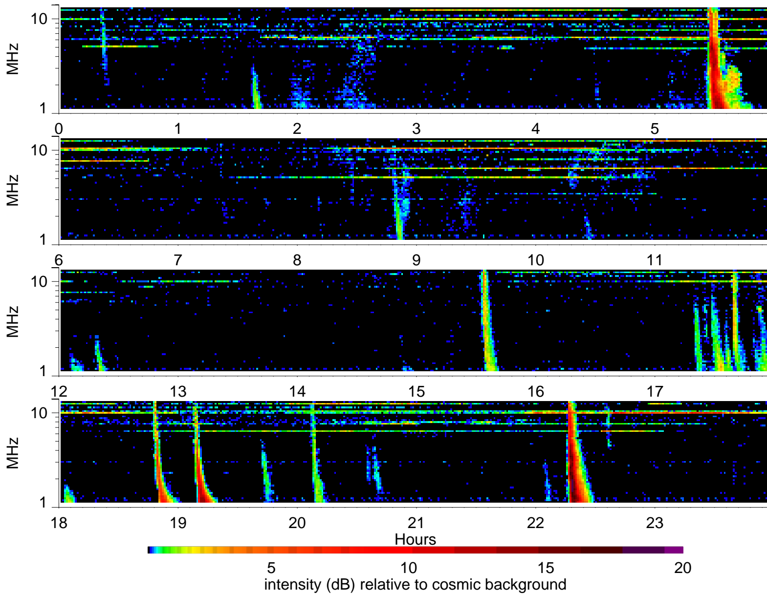
Wind Waves RAD2 receiver: 2001/3/12
