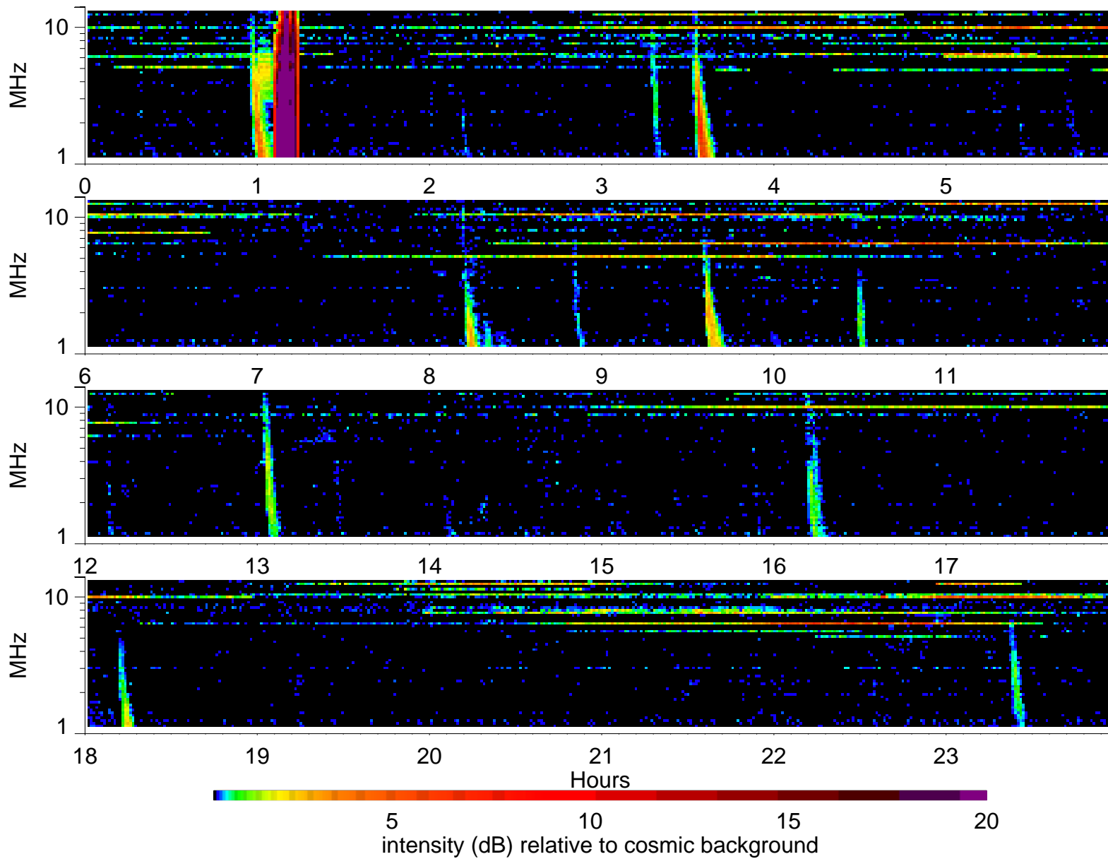
Wind Waves RAD2 receiver: 2001/3/11
