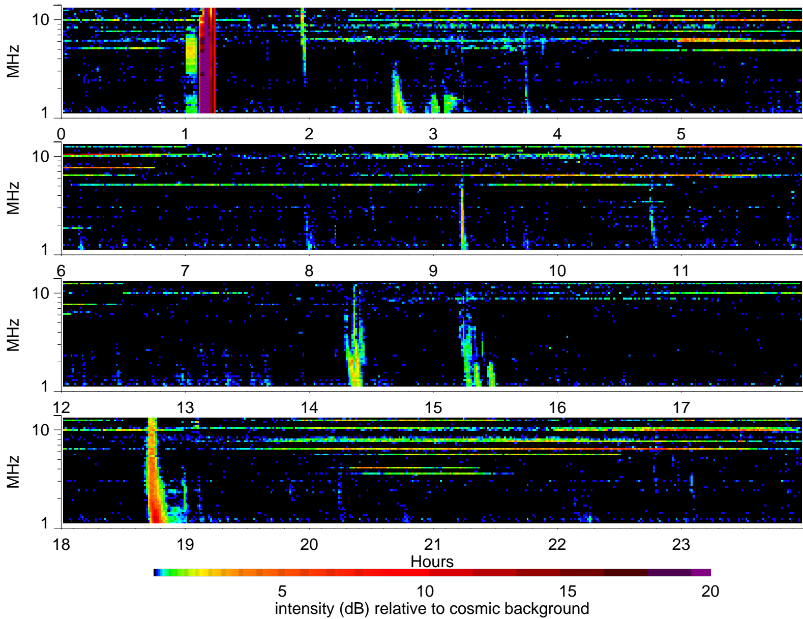
Wind Waves RAD2 receiver: 2001/3/9
