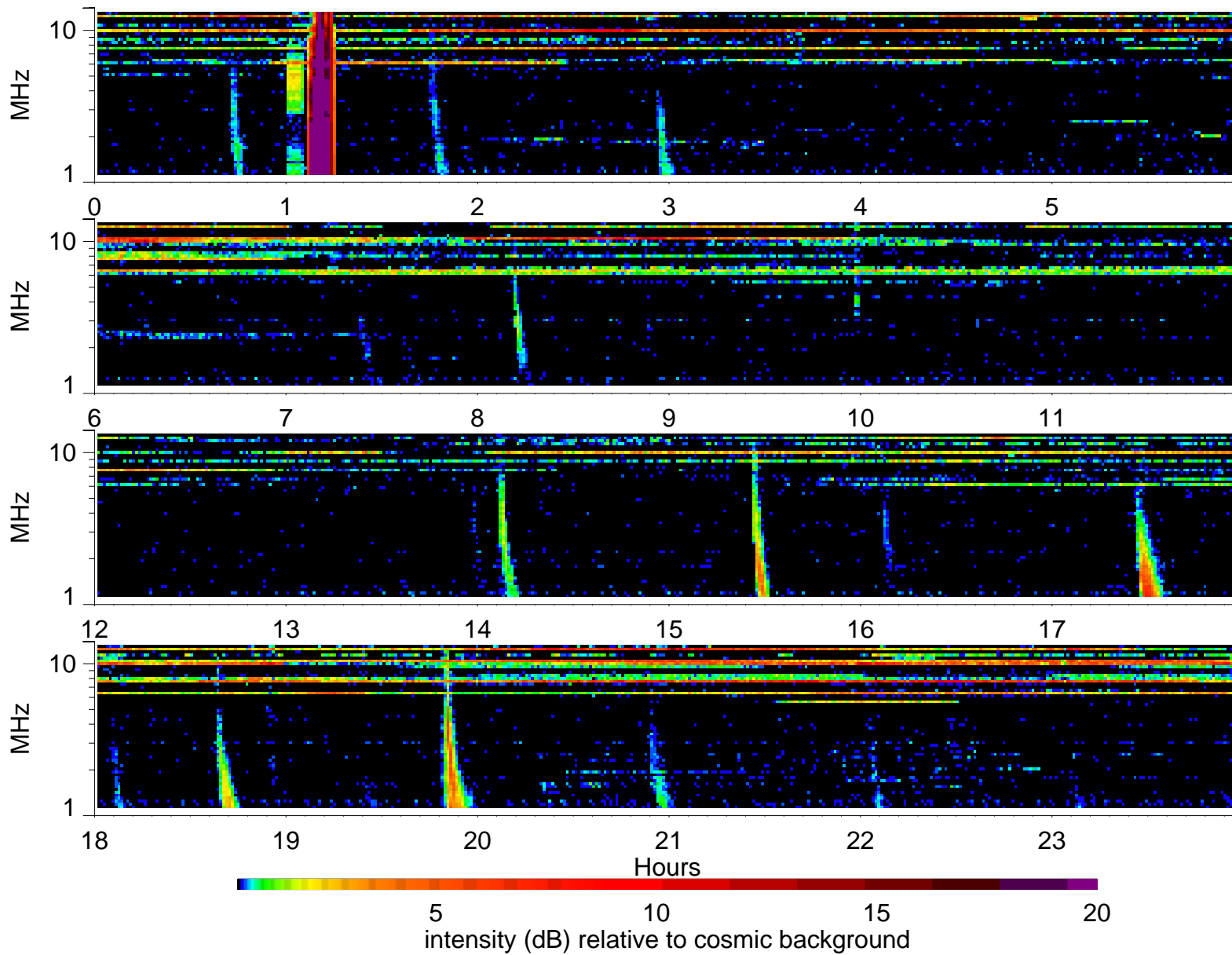
Wind Waves RAD2 receiver: 2001/2/27
