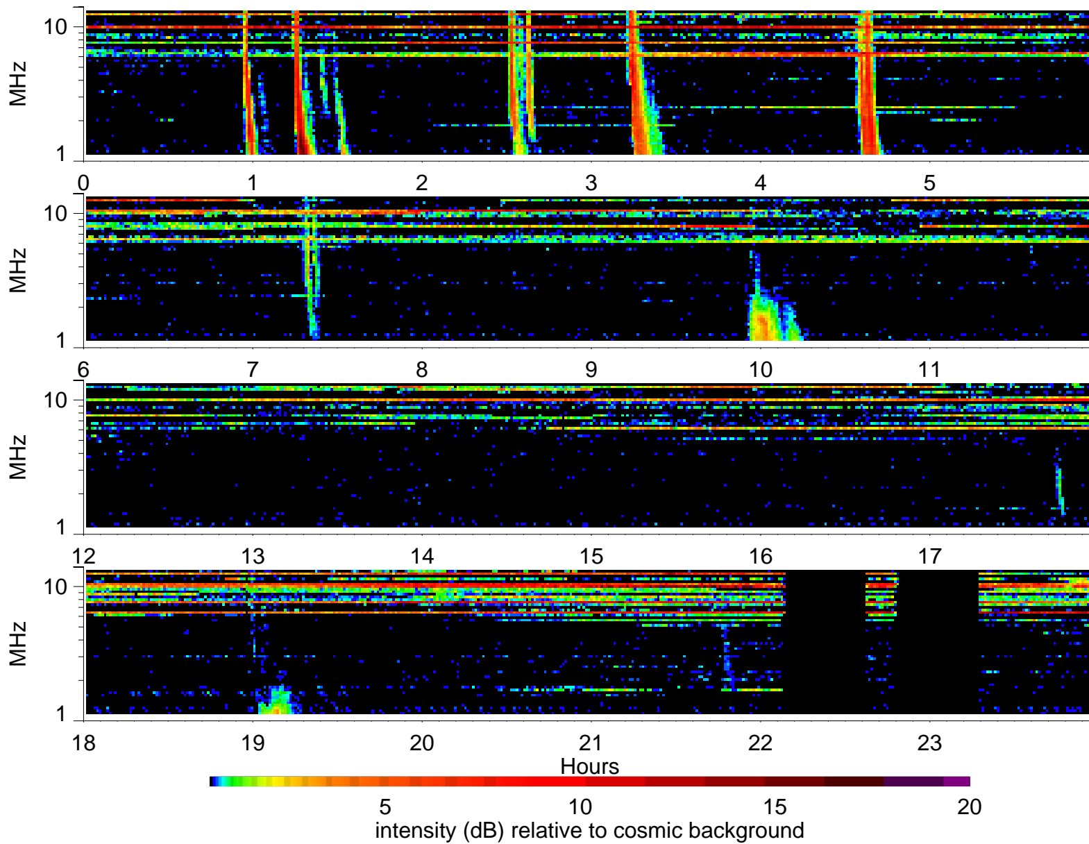
Wind Waves RAD2 receiver: 2001/2/24
