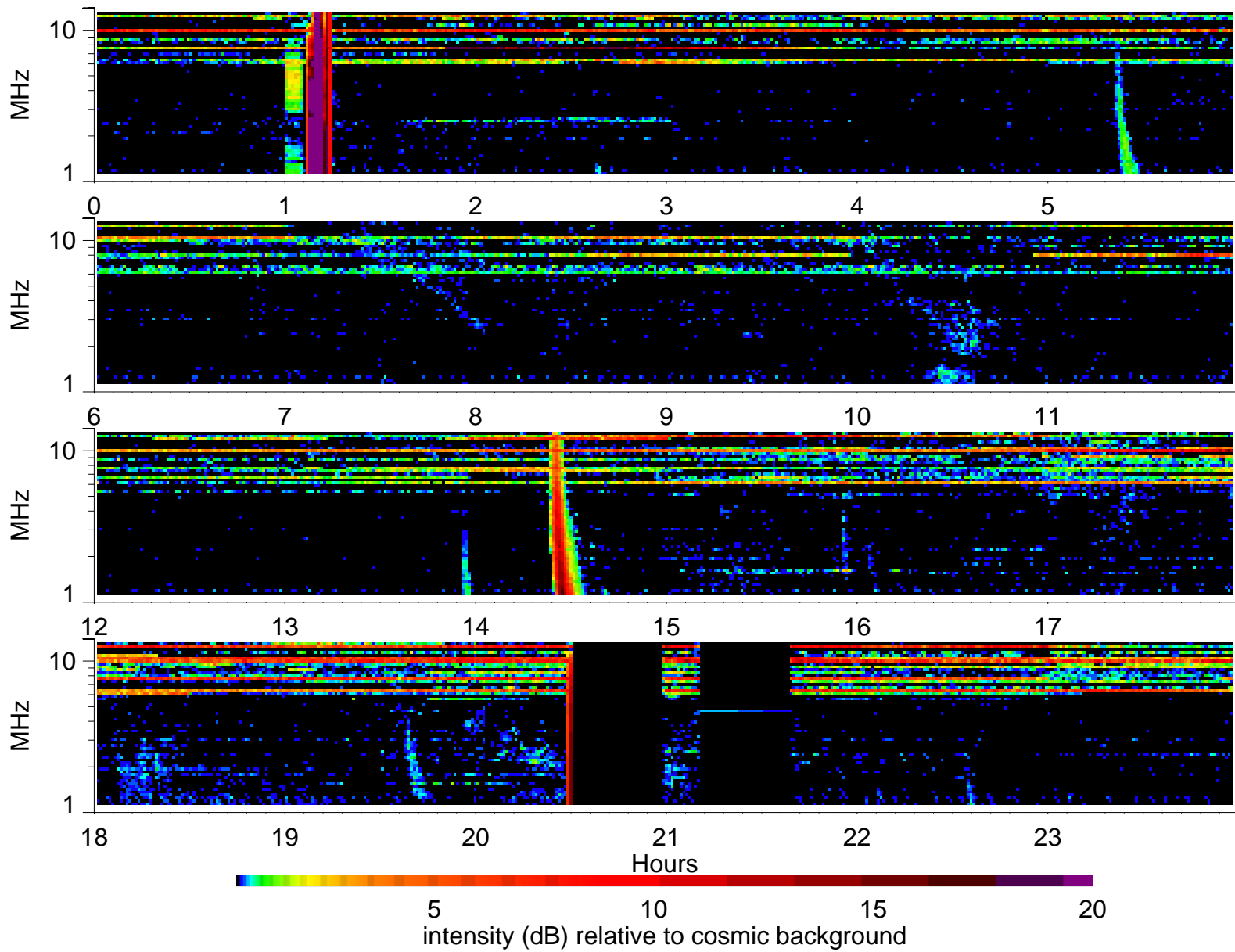
Wind Waves RAD2 receiver: 2001/2/21
