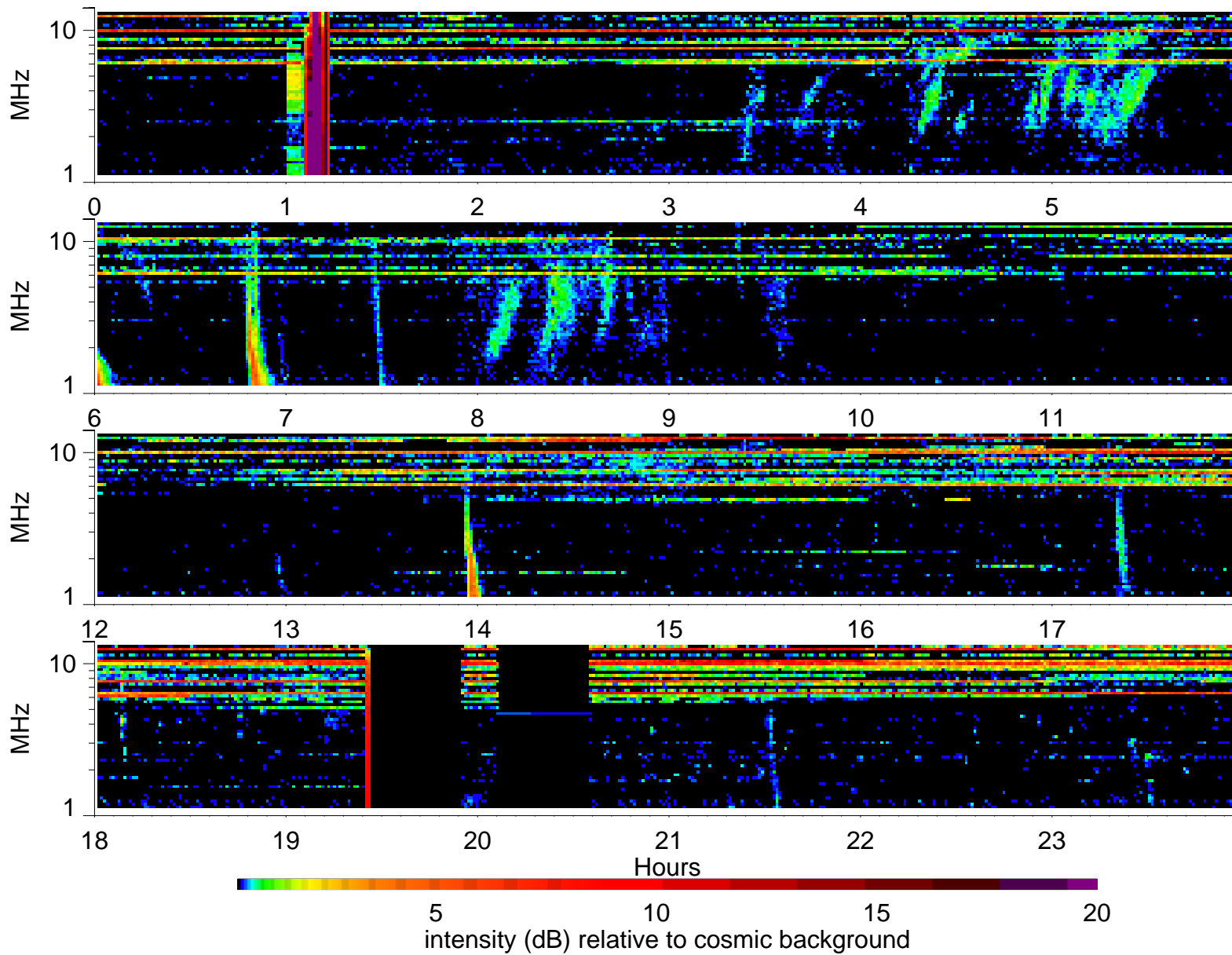
Wind Waves RAD2 receiver: 2001/2/19
