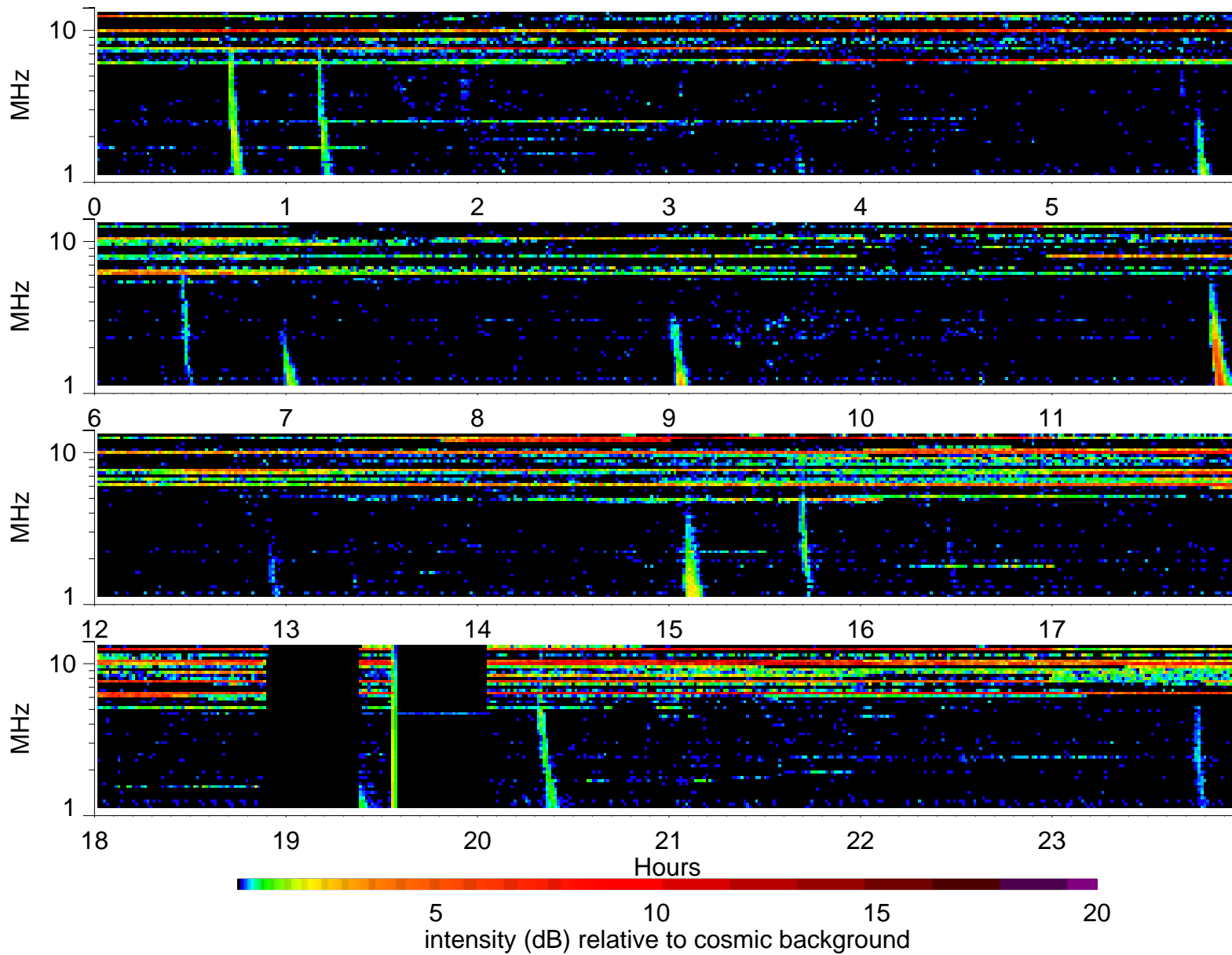
Wind Waves RAD2 receiver: 2001/2/18
