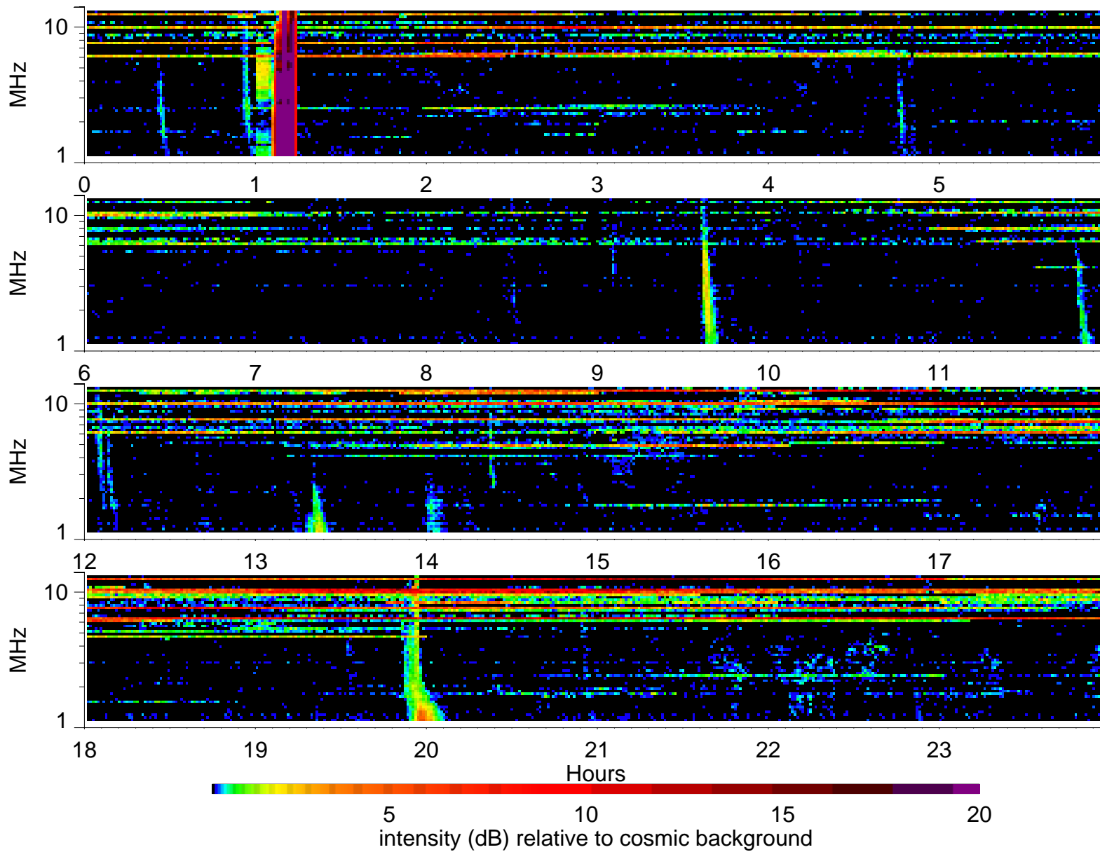
Wind Waves RAD2 receiver: 2001/2/15
