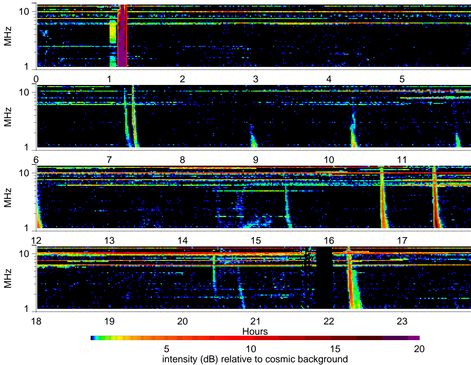
Wind Waves RAD2 receiver: 2001/2/13
