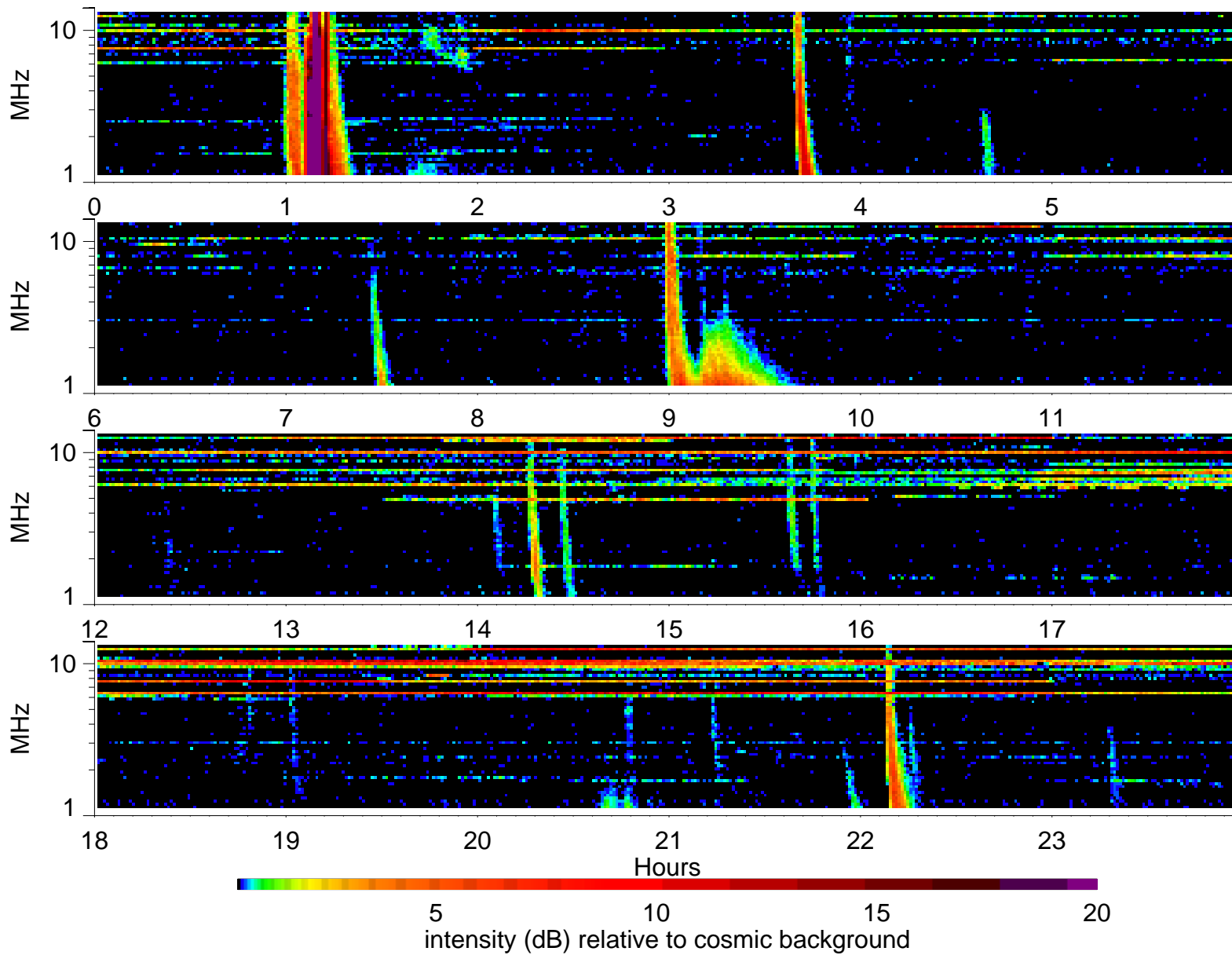
Wind Waves RAD2 receiver: 2001/2/11
