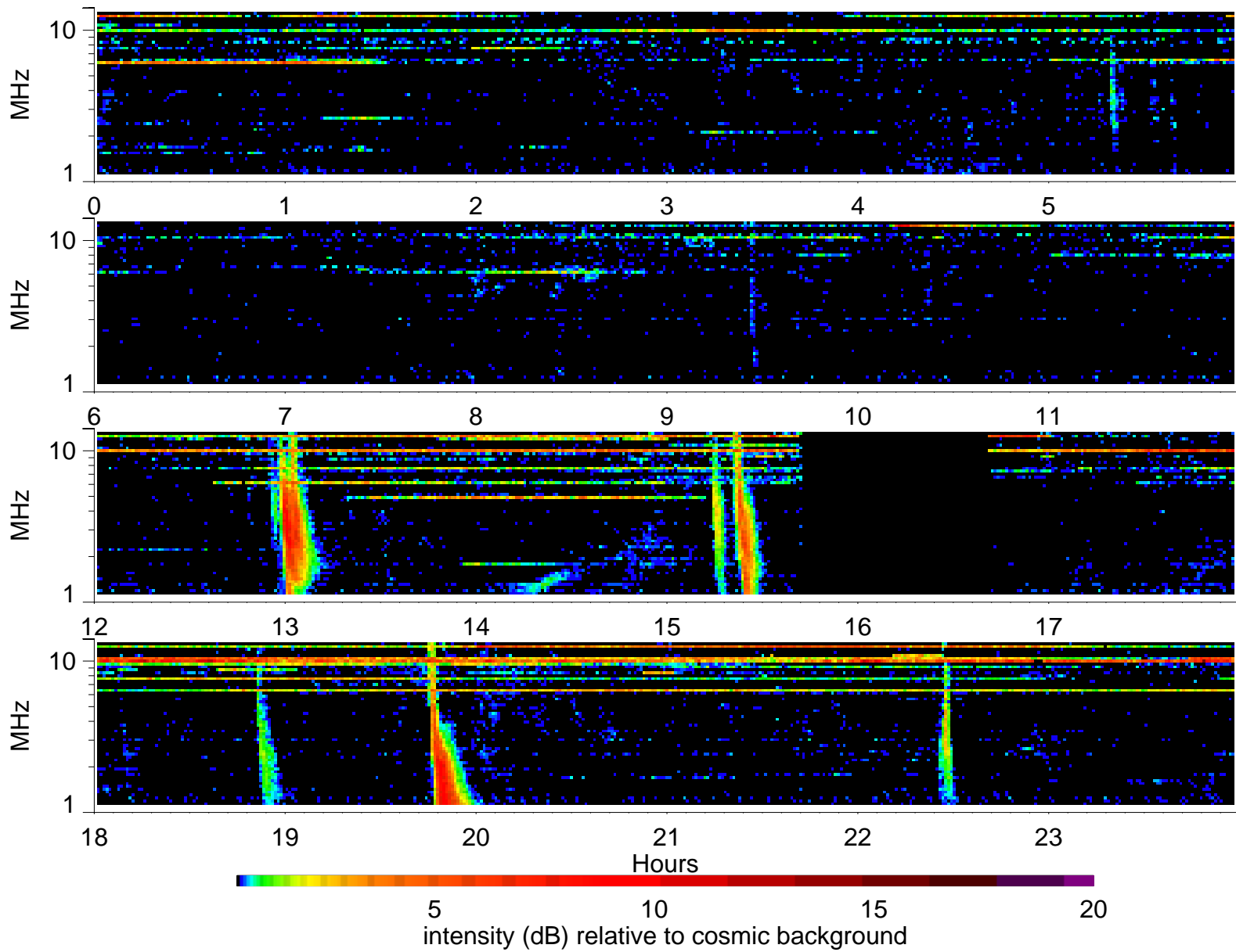
Wind Waves RAD2 receiver: 2001/2/6
