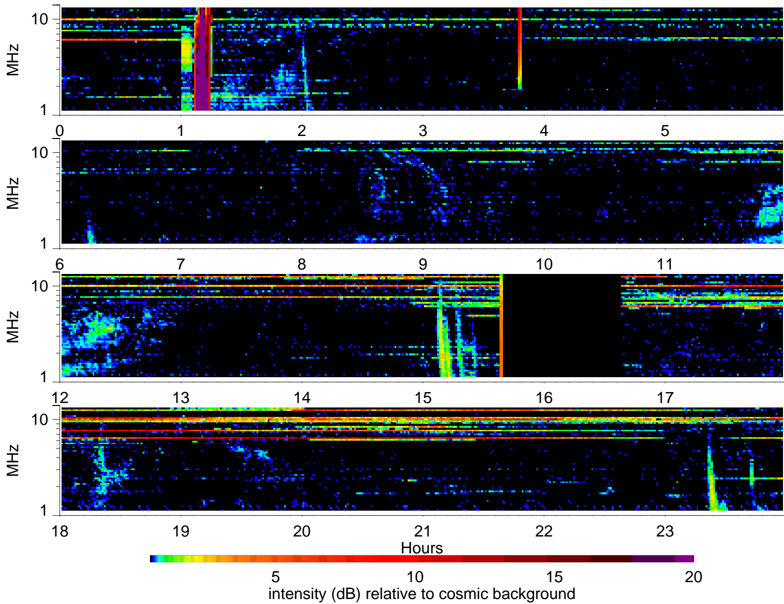
Wind Waves RAD2 receiver: 2001/2/5
