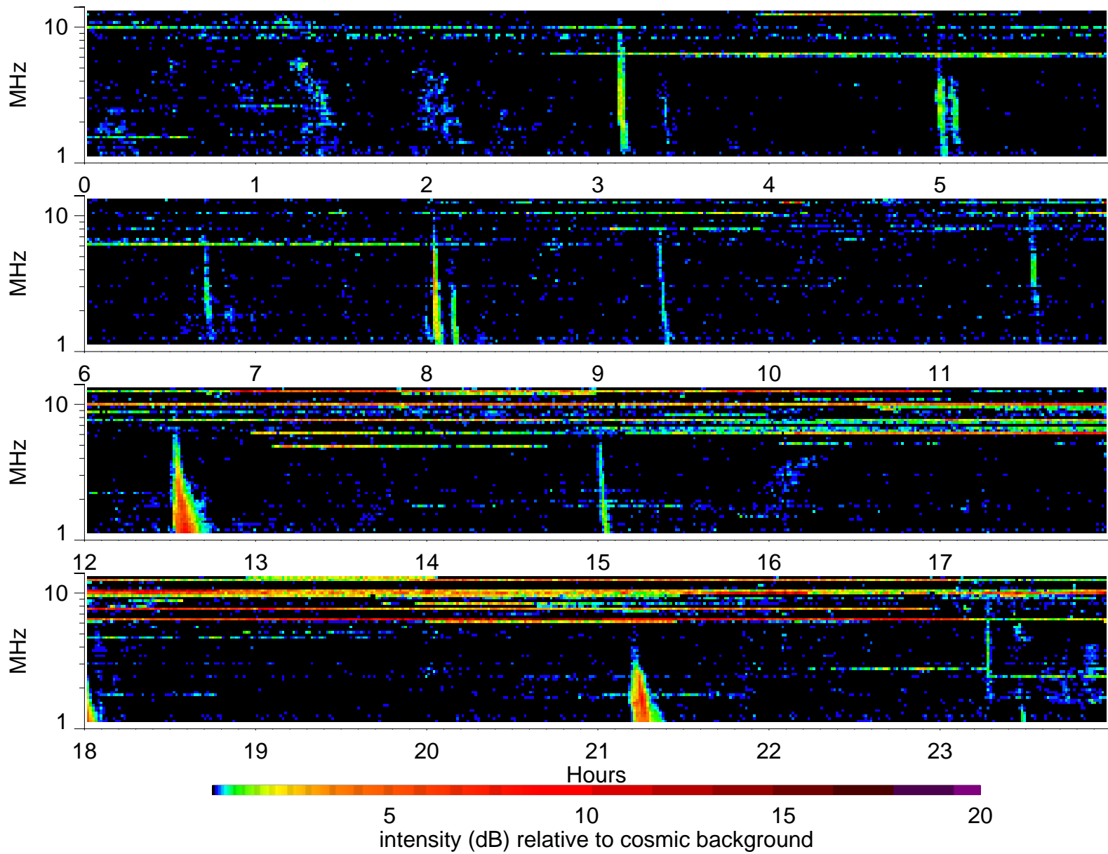
Wind Waves RAD2 receiver: 2001/2/4
