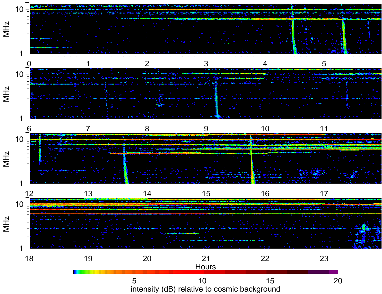
Wind Waves RAD2 receiver: 2001/1/31
