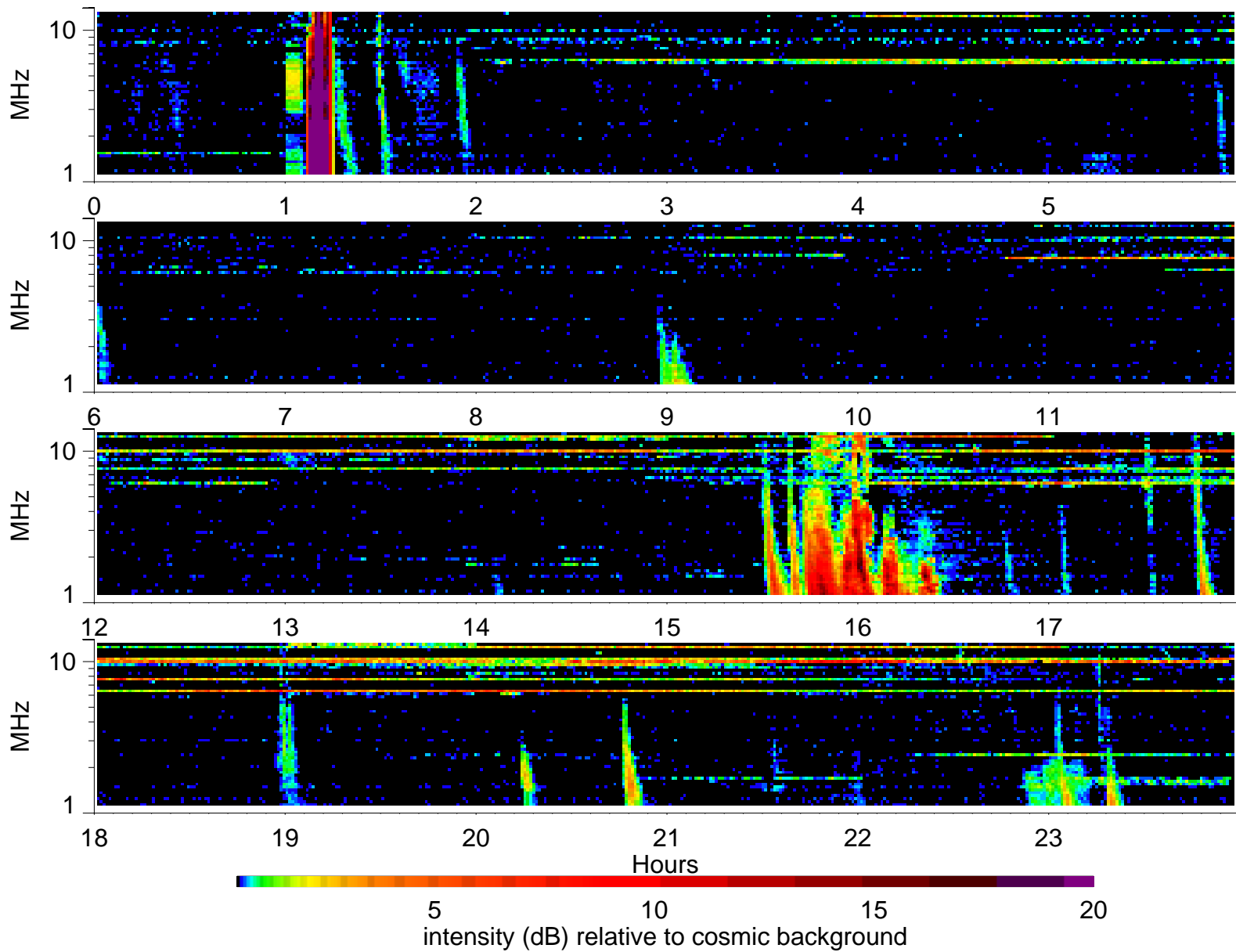
Wind Waves RAD2 receiver: 2001/1/28
