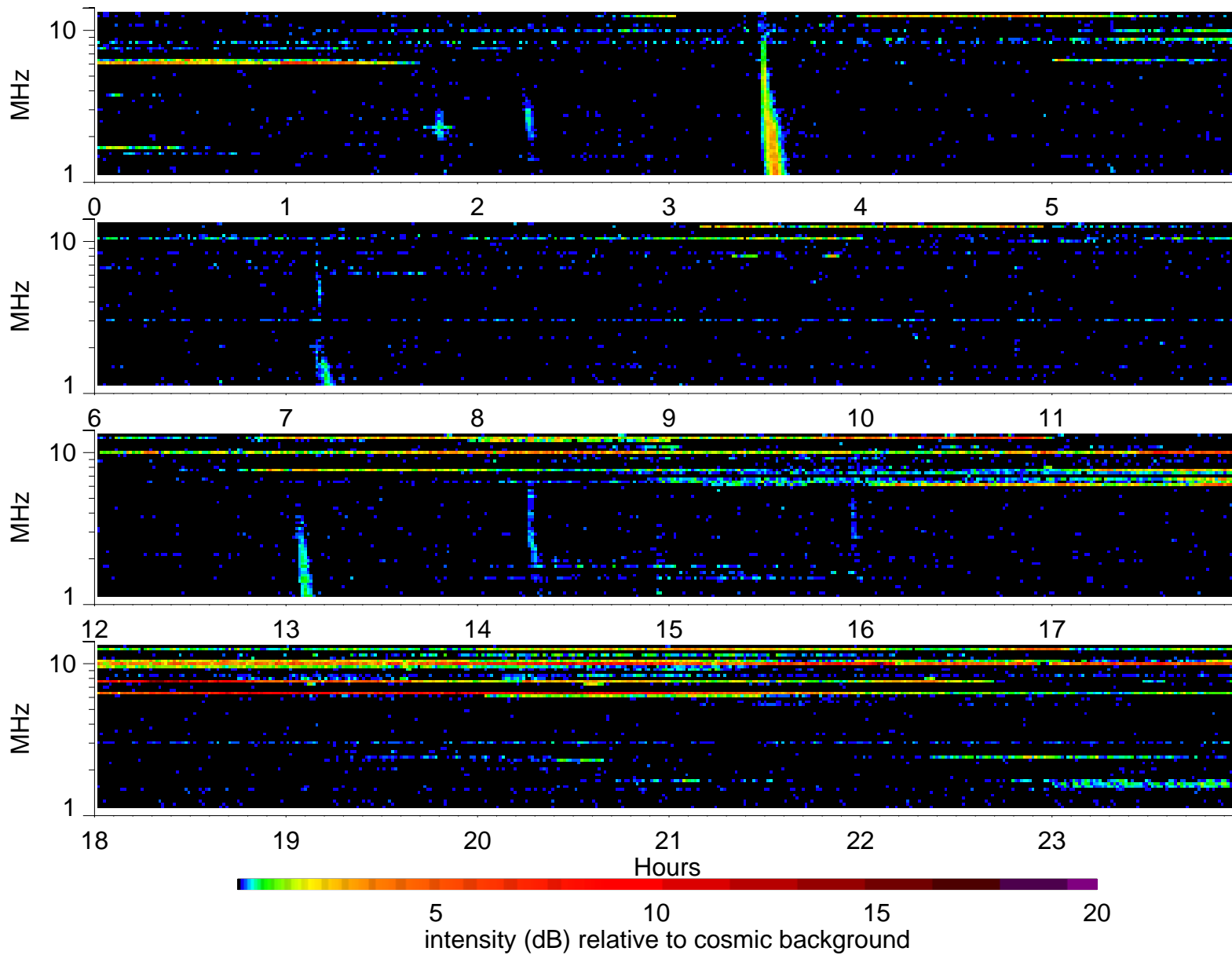
Wind Waves RAD2 receiver: 2001/1/25
