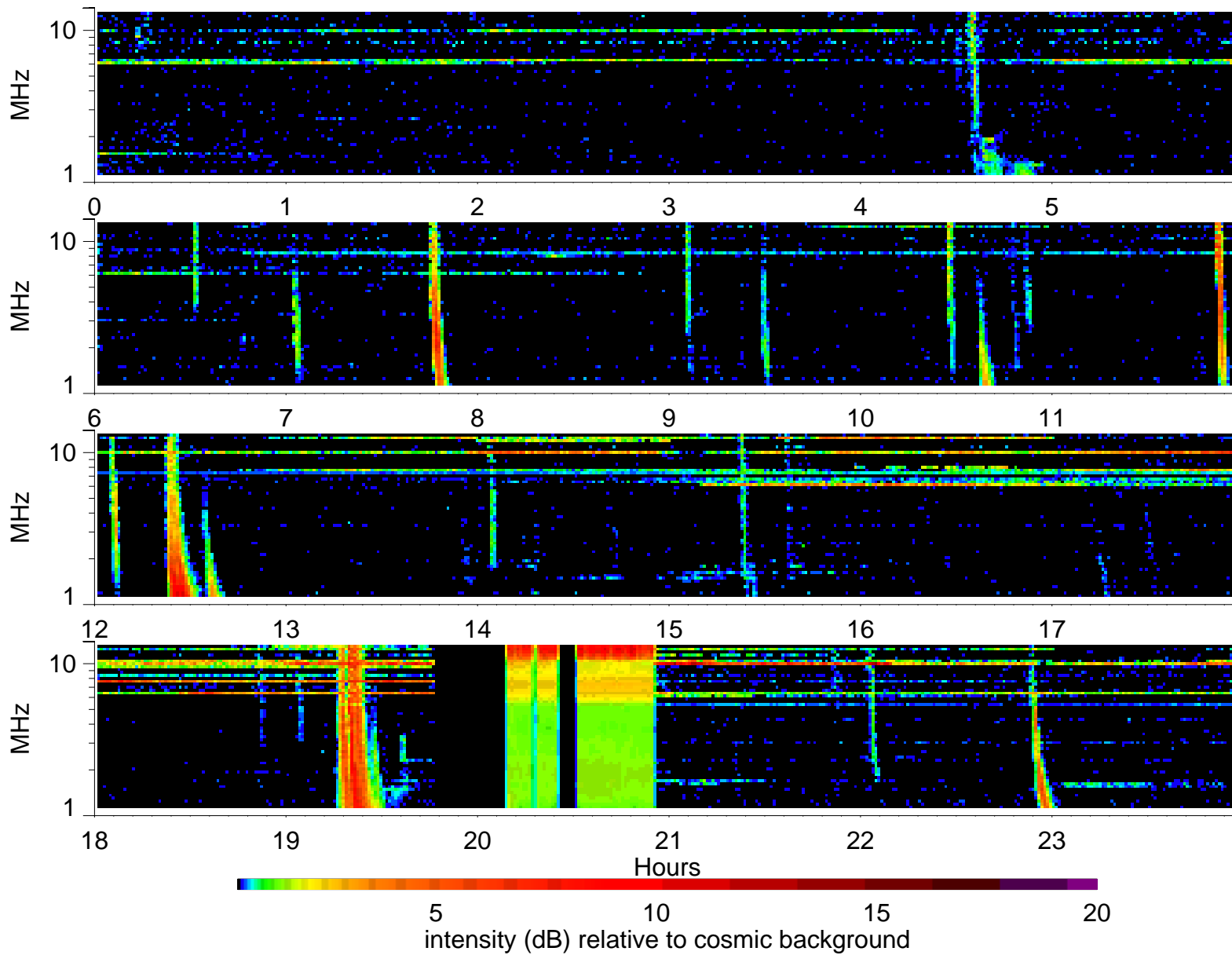
Wind Waves RAD2 receiver: 2001/1/21
