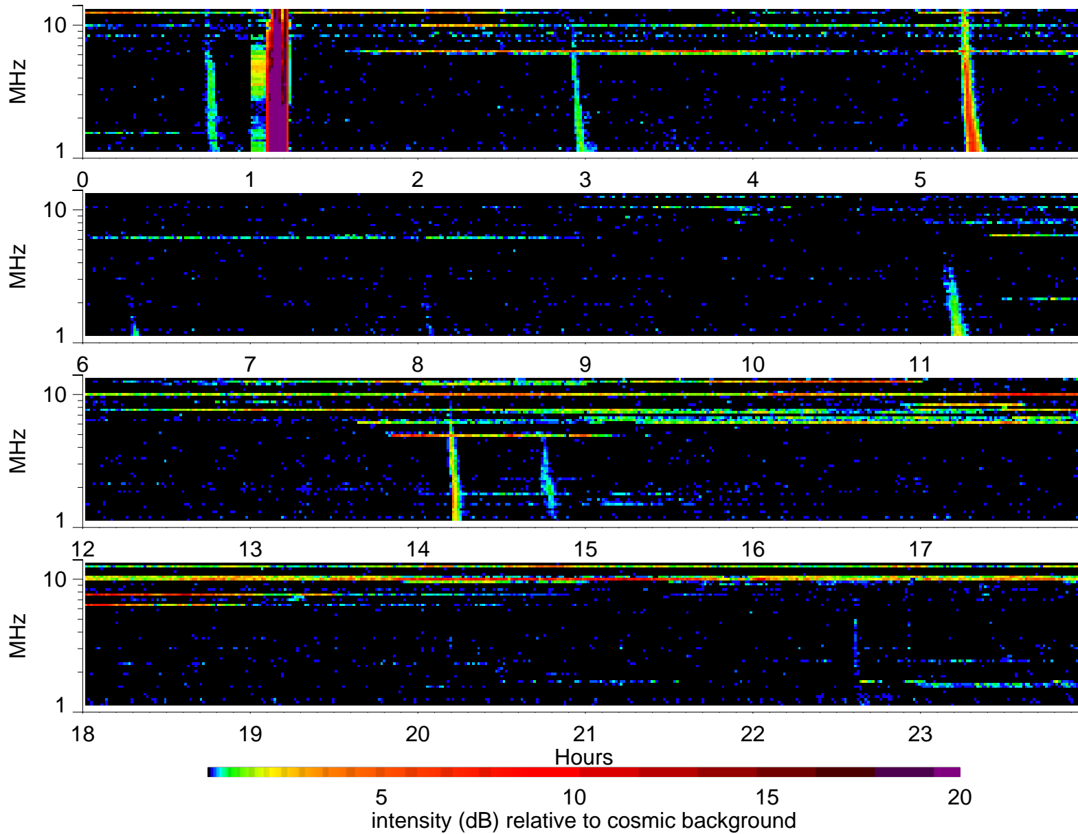
Wind Waves RAD2 receiver: 2001/1/18
