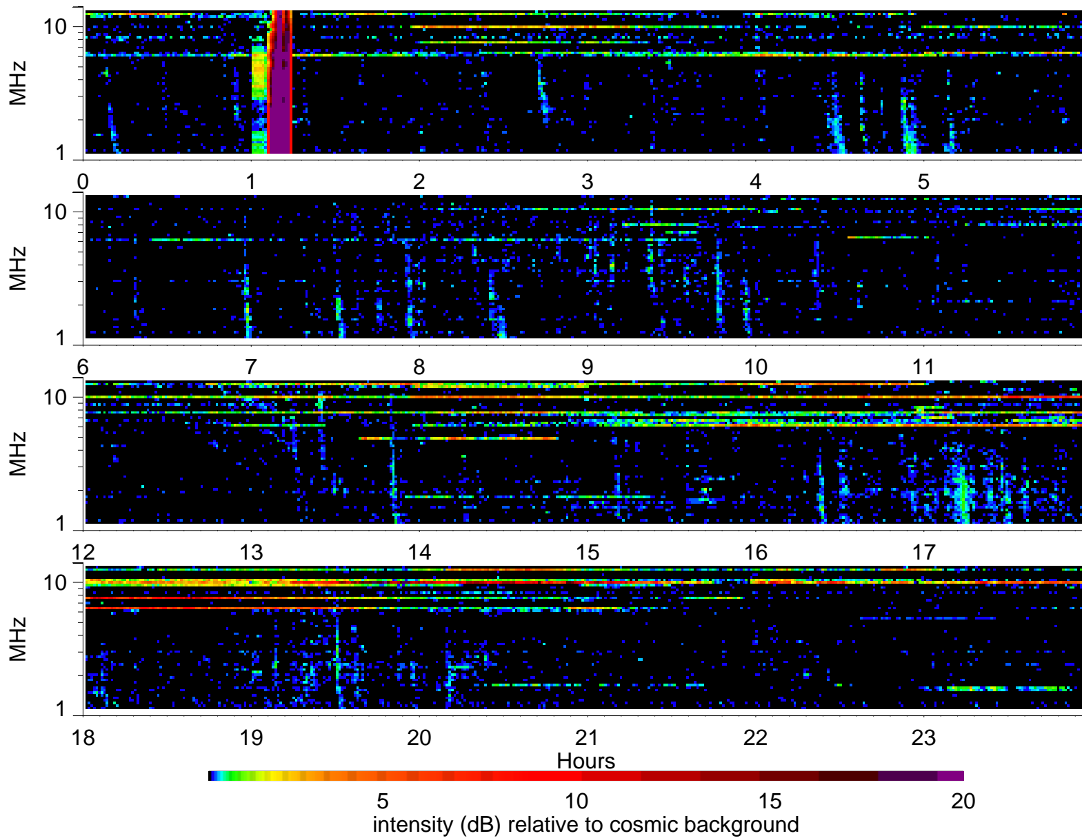
Wind Waves RAD2 receiver: 2001/1/16
