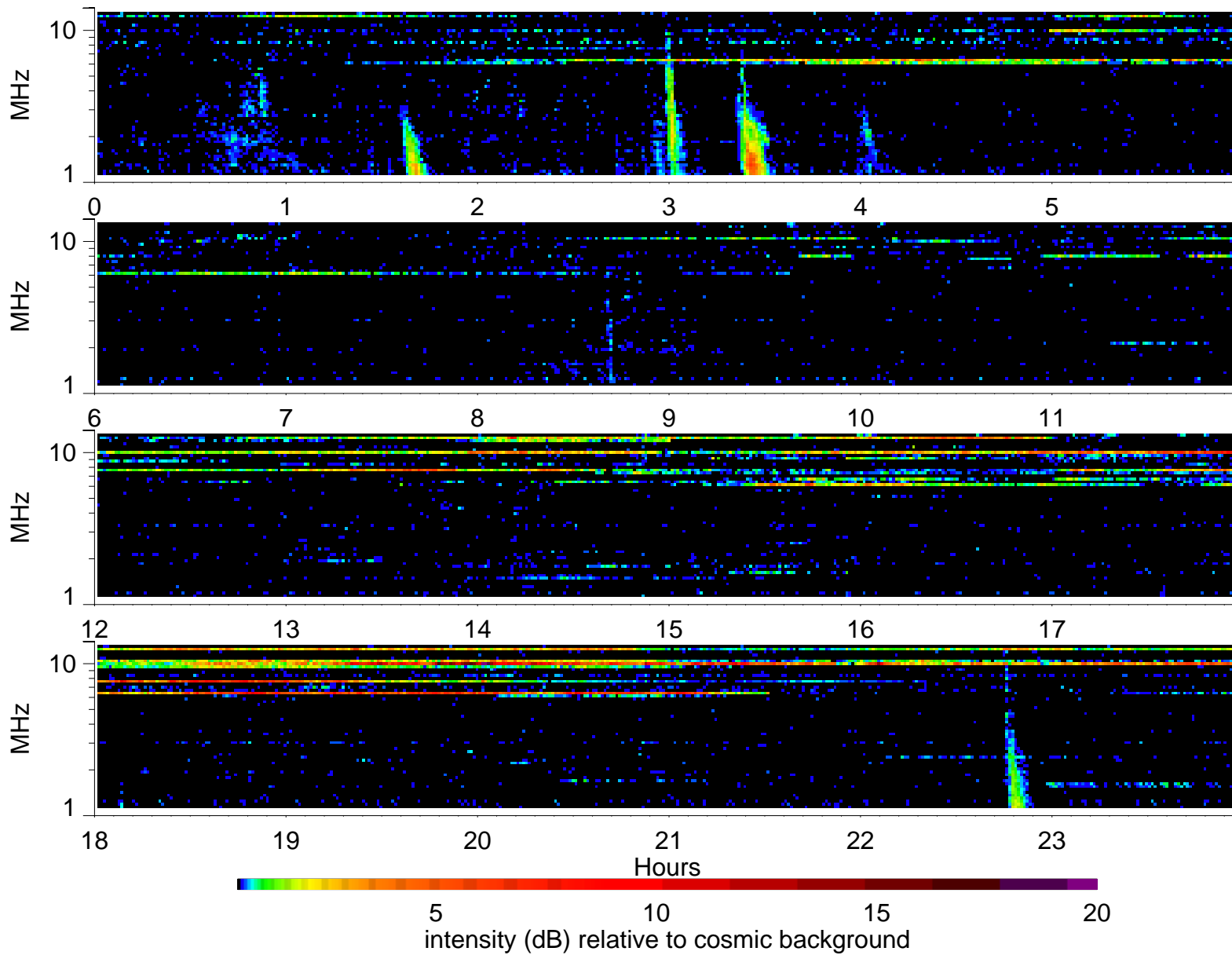
Wind Waves RAD2 receiver: 2001/1/13
