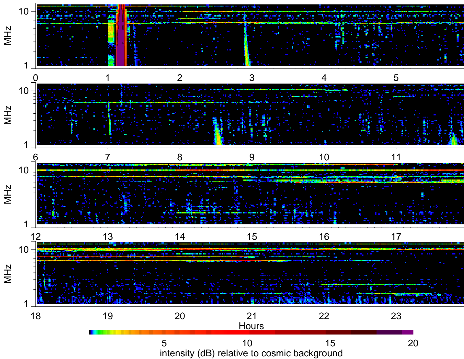
Wind Waves RAD2 receiver: 2001/1/12
