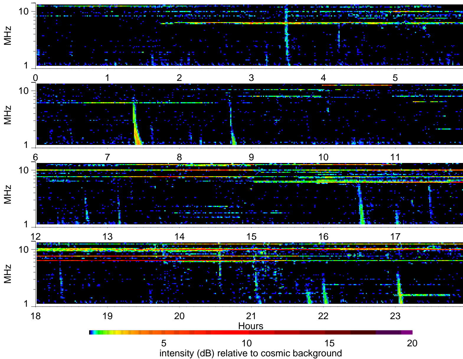
Wind Waves RAD2 receiver: 2001/1/11
