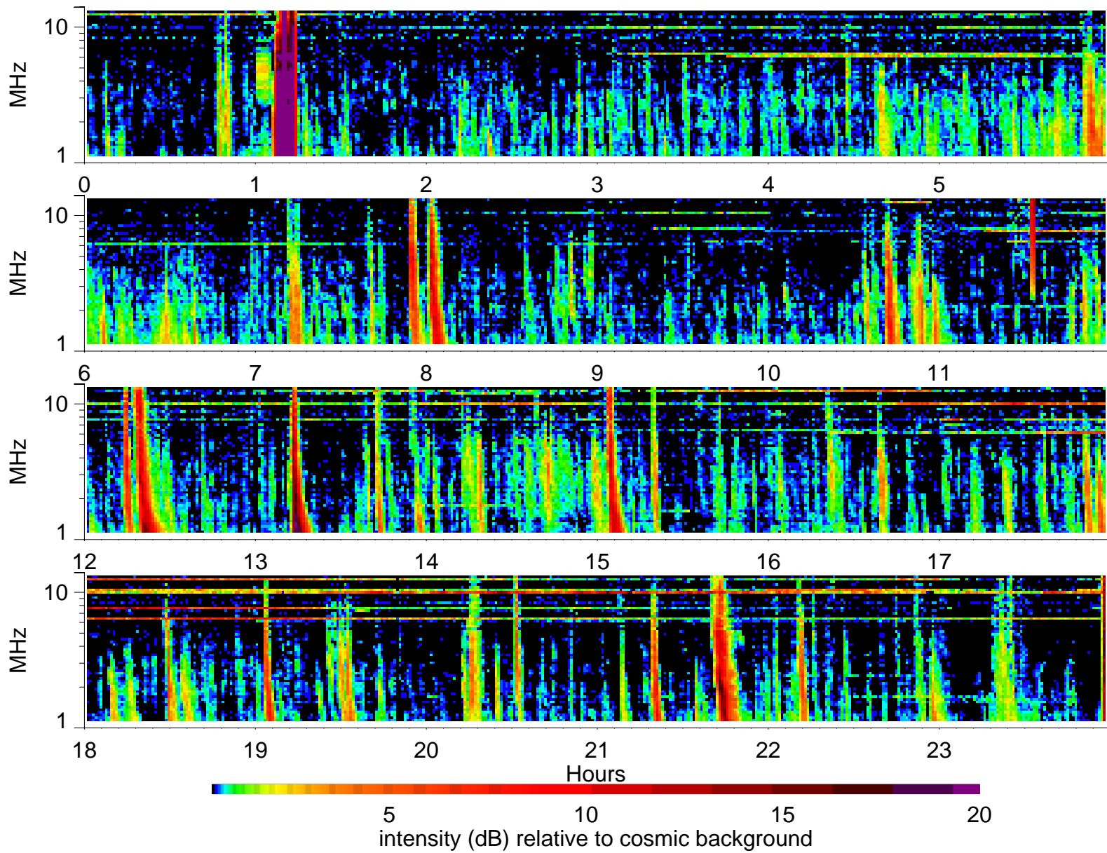
Wind Waves RAD2 receiver: 2001/1/8
