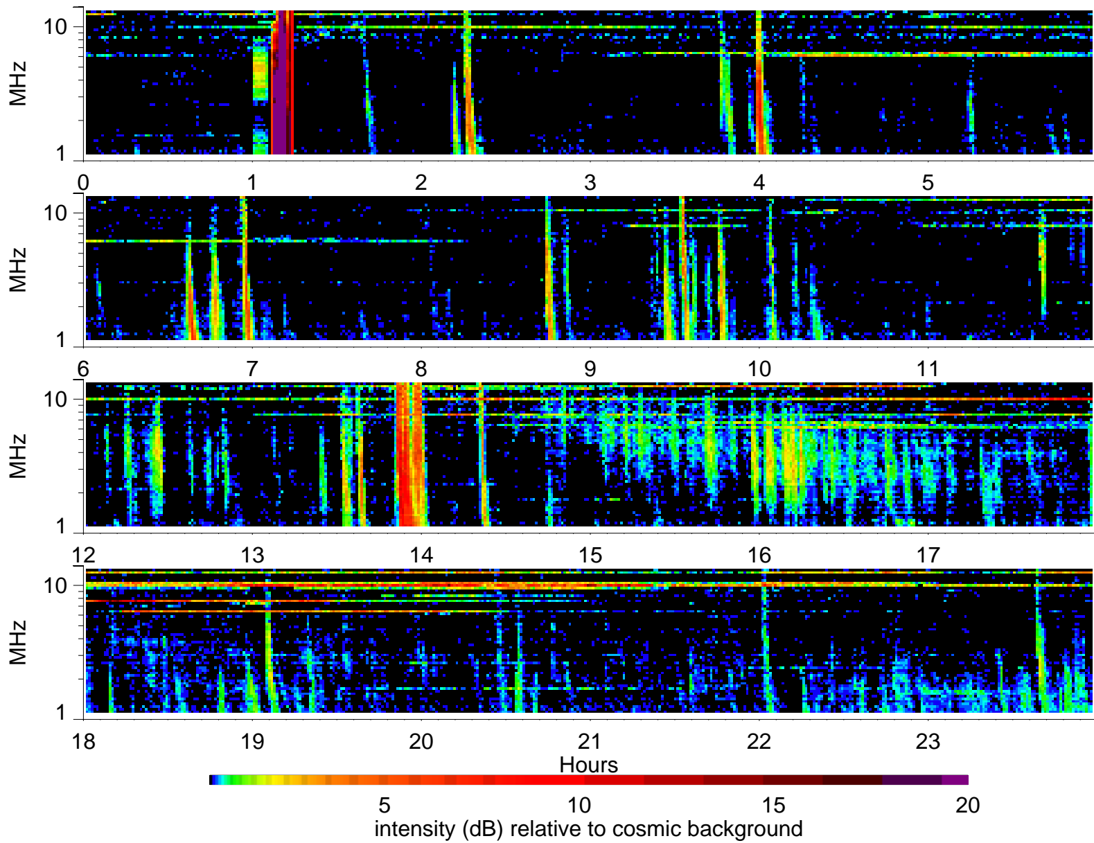
Wind Waves RAD2 receiver: 2001/1/6
