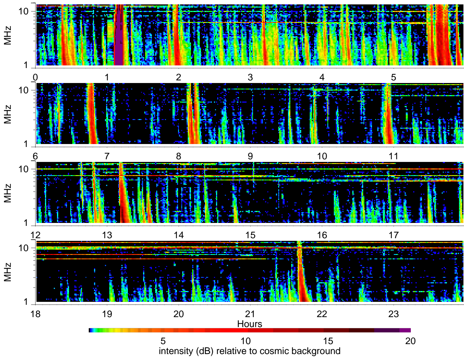
Wind Waves RAD2 receiver: 2001/1/2
