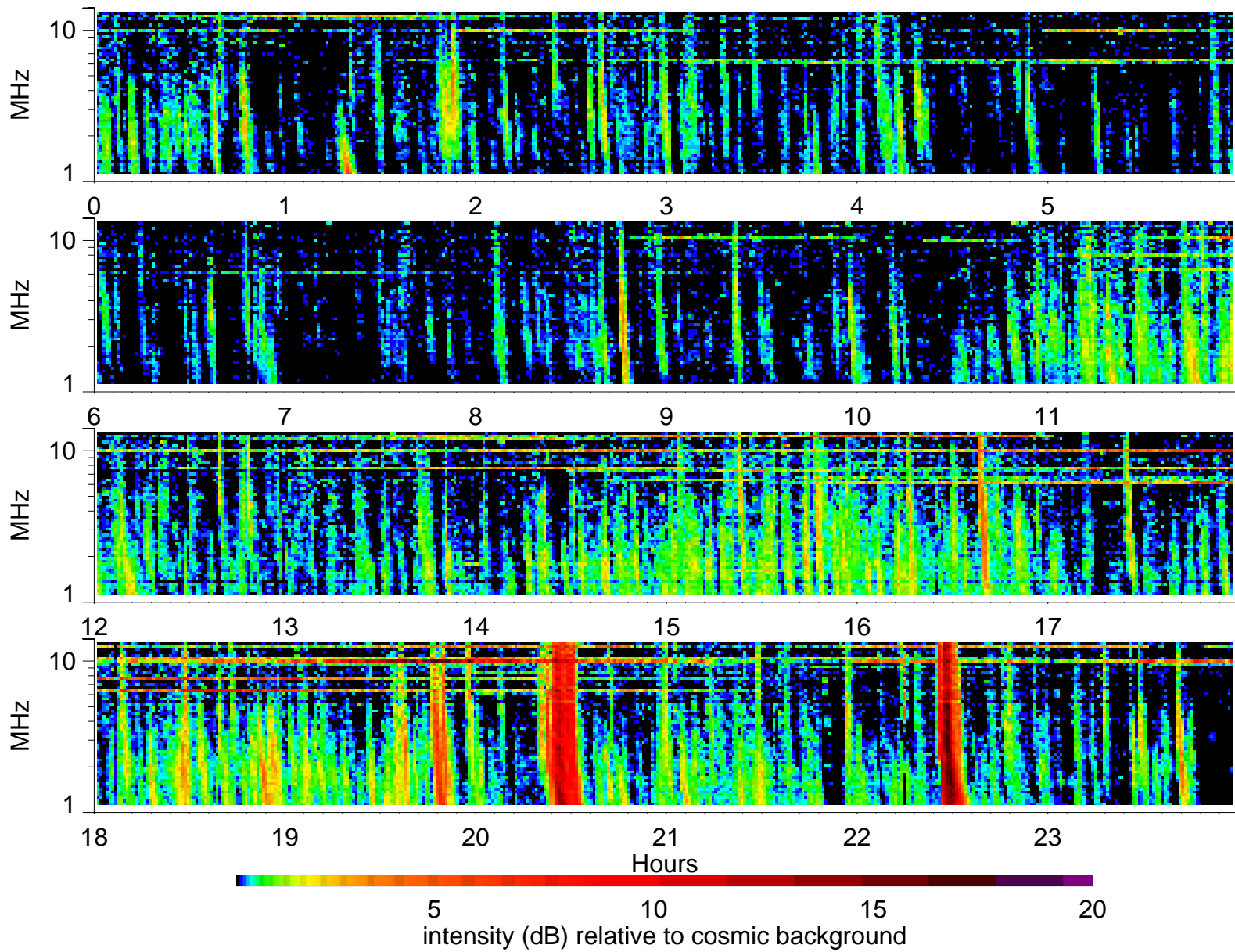
Wind Waves RAD2 receiver: 2001/1/1
