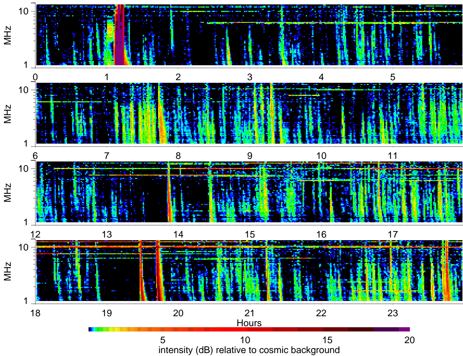
Wind Waves RAD2 receiver: 2000/12/31
