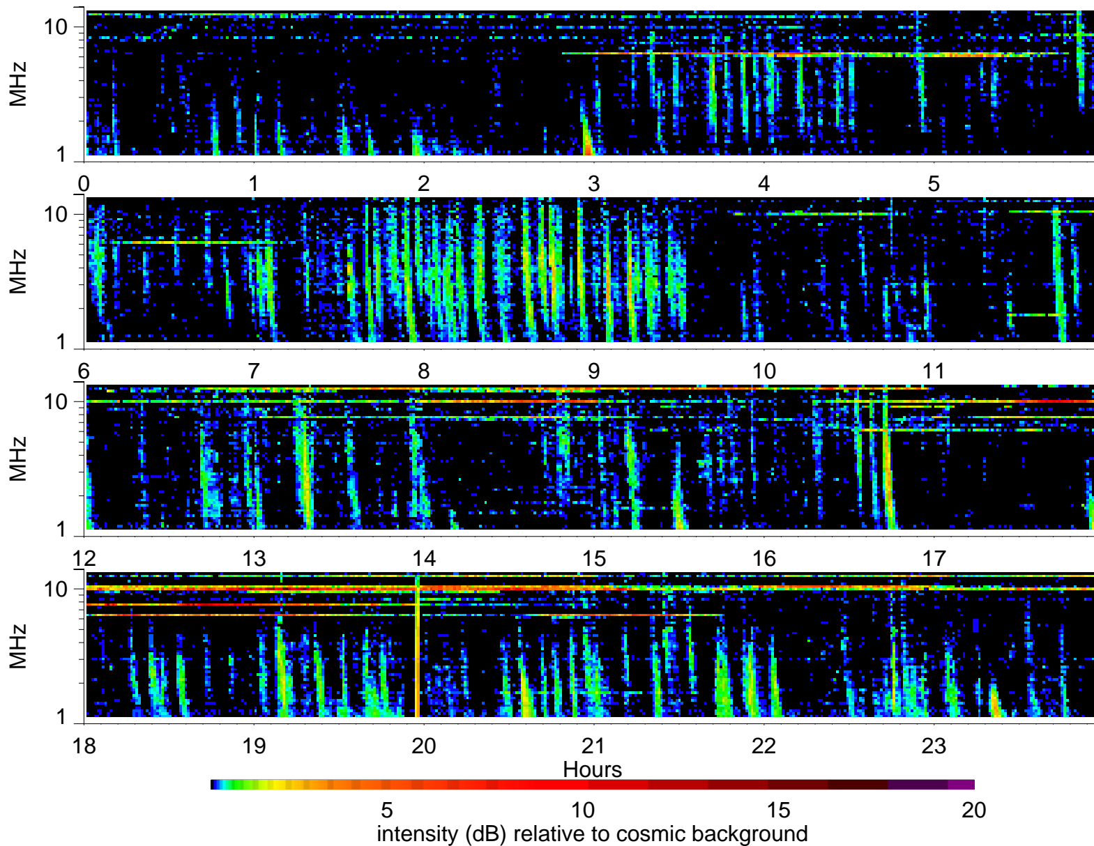
Wind Waves RAD2 receiver: 2000/12/30
