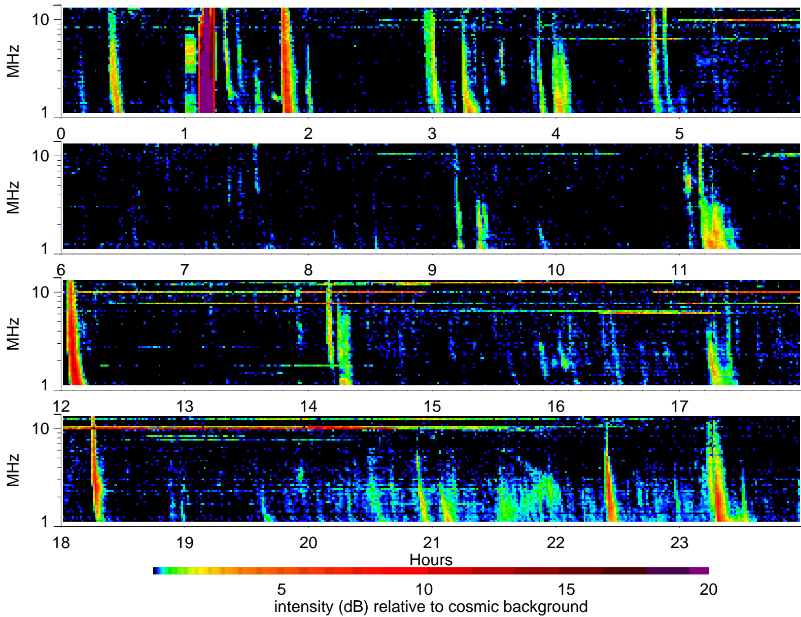
Wind Waves RAD2 receiver: 2000/12/21
