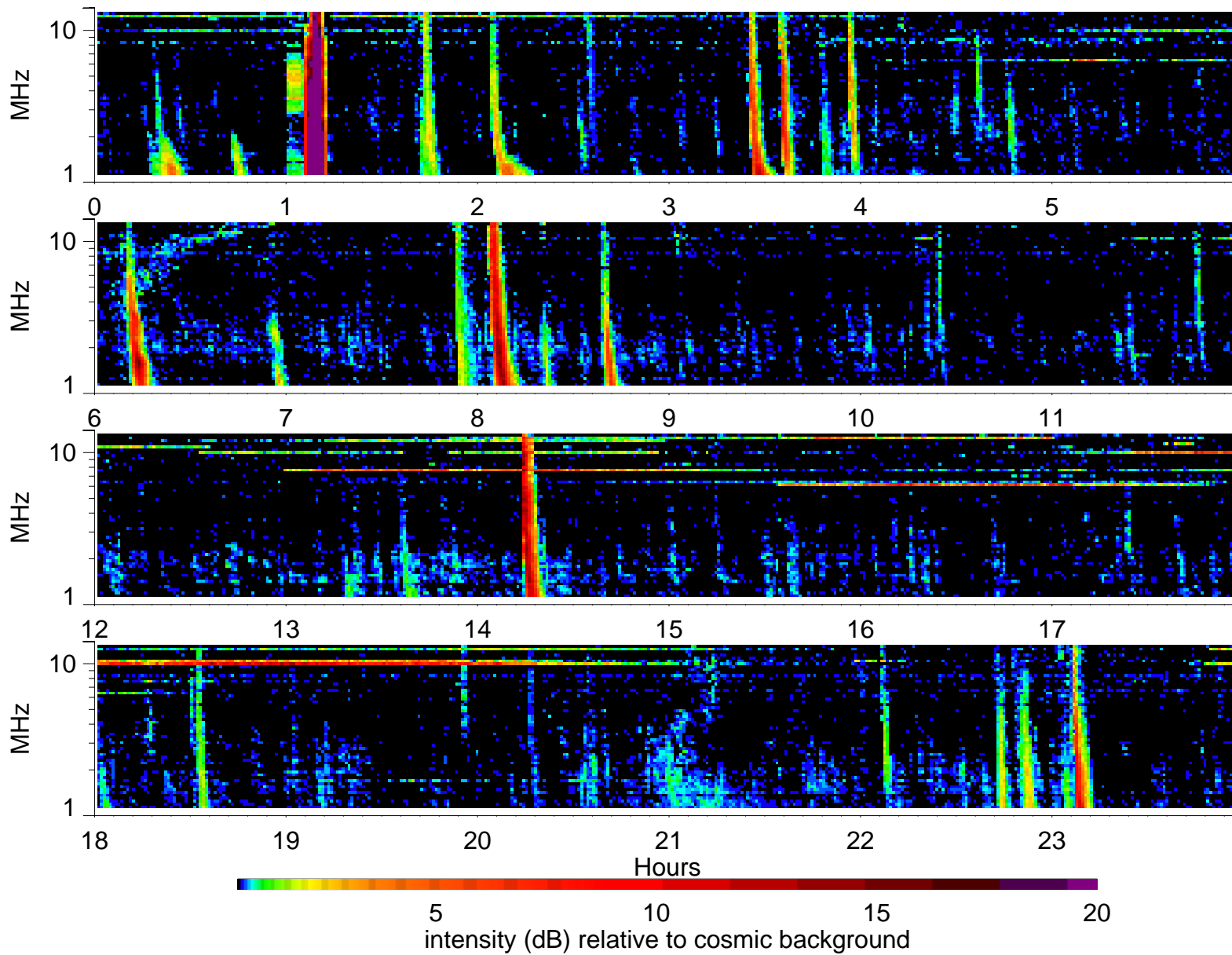
Wind Waves RAD2 receiver: 2000/12/19
