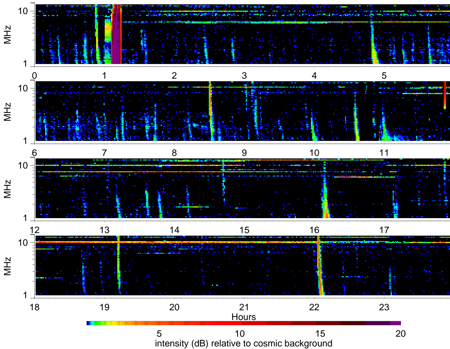
Wind Waves RAD2 receiver: 2000/12/17
