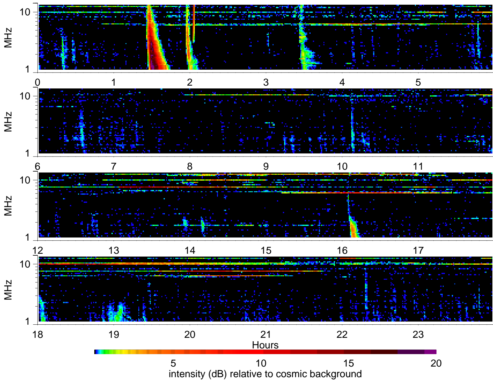
Wind Waves RAD2 receiver: 2000/12/16
