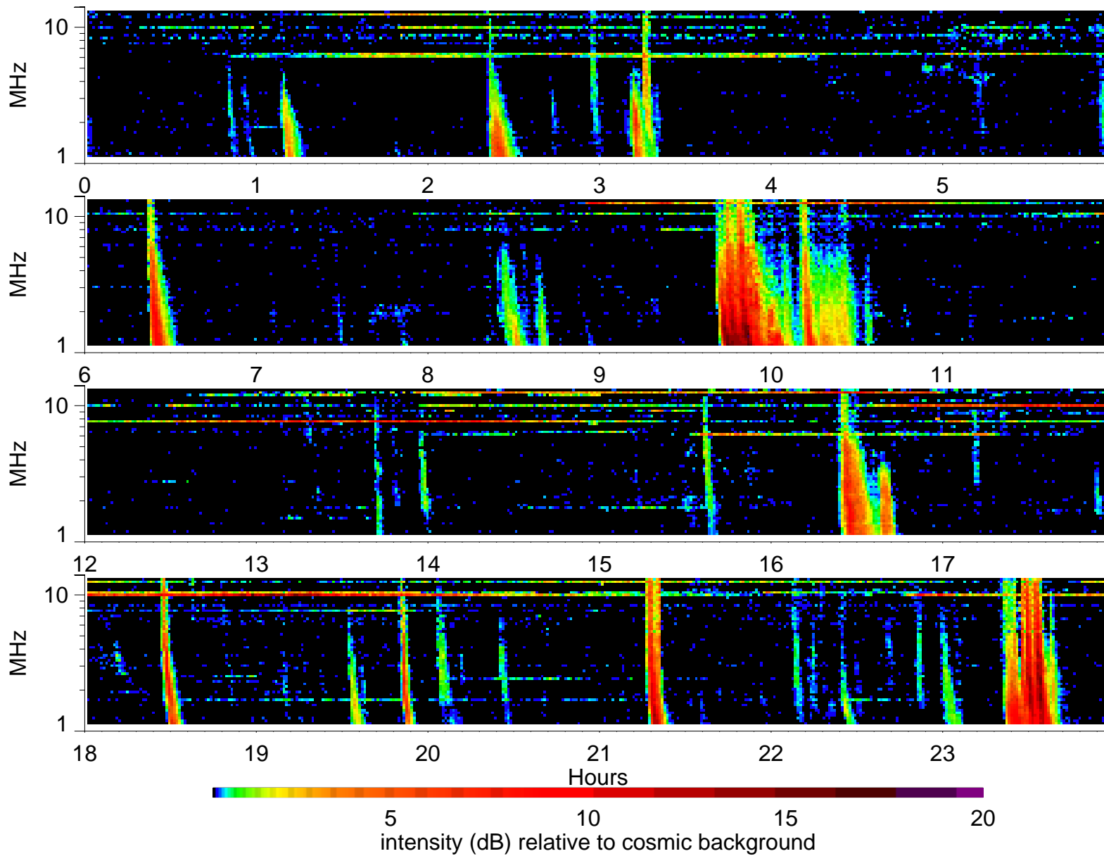
Wind Waves RAD2 receiver: 2000/12/14
