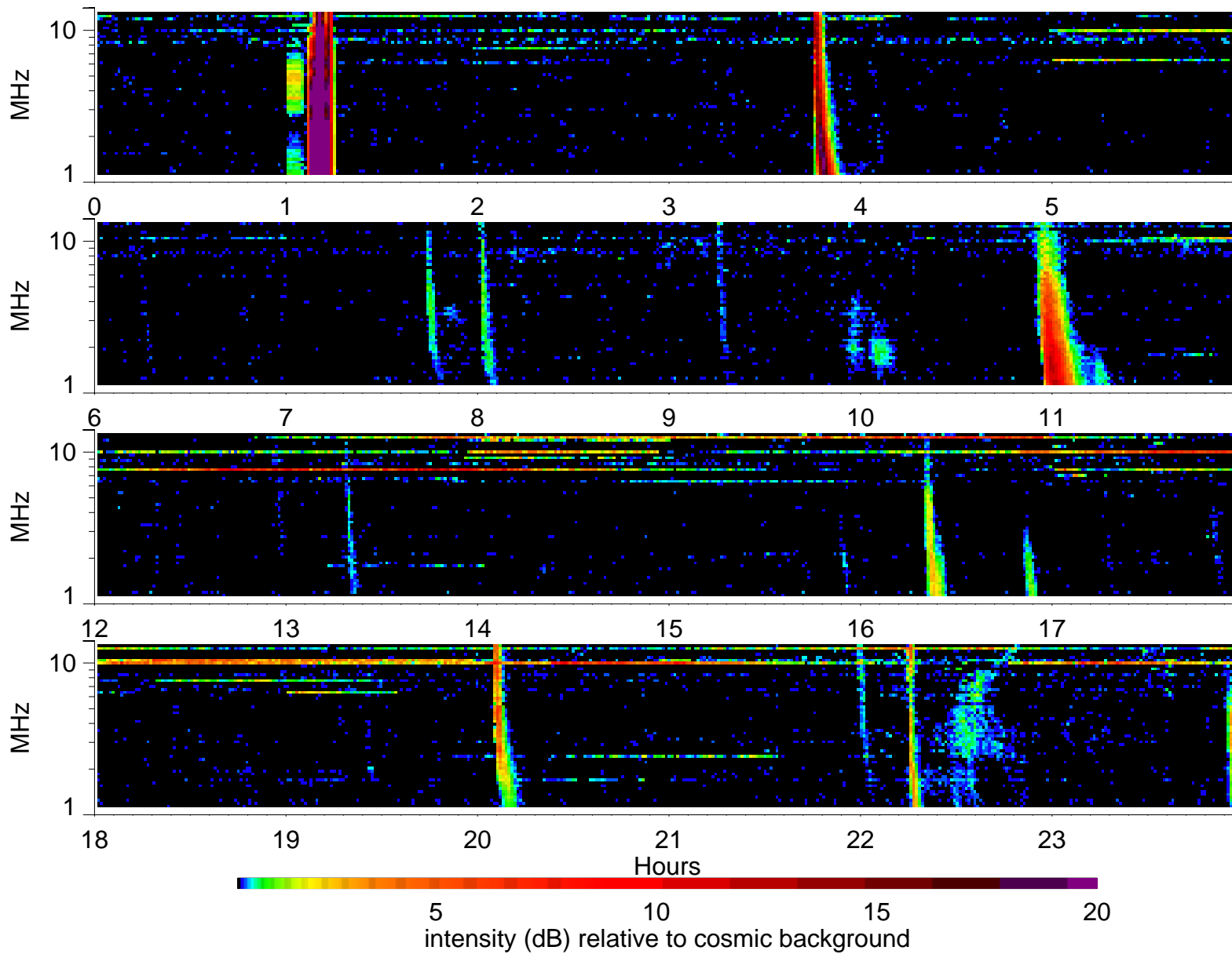
Wind Waves RAD2 receiver: 2000/12/13
