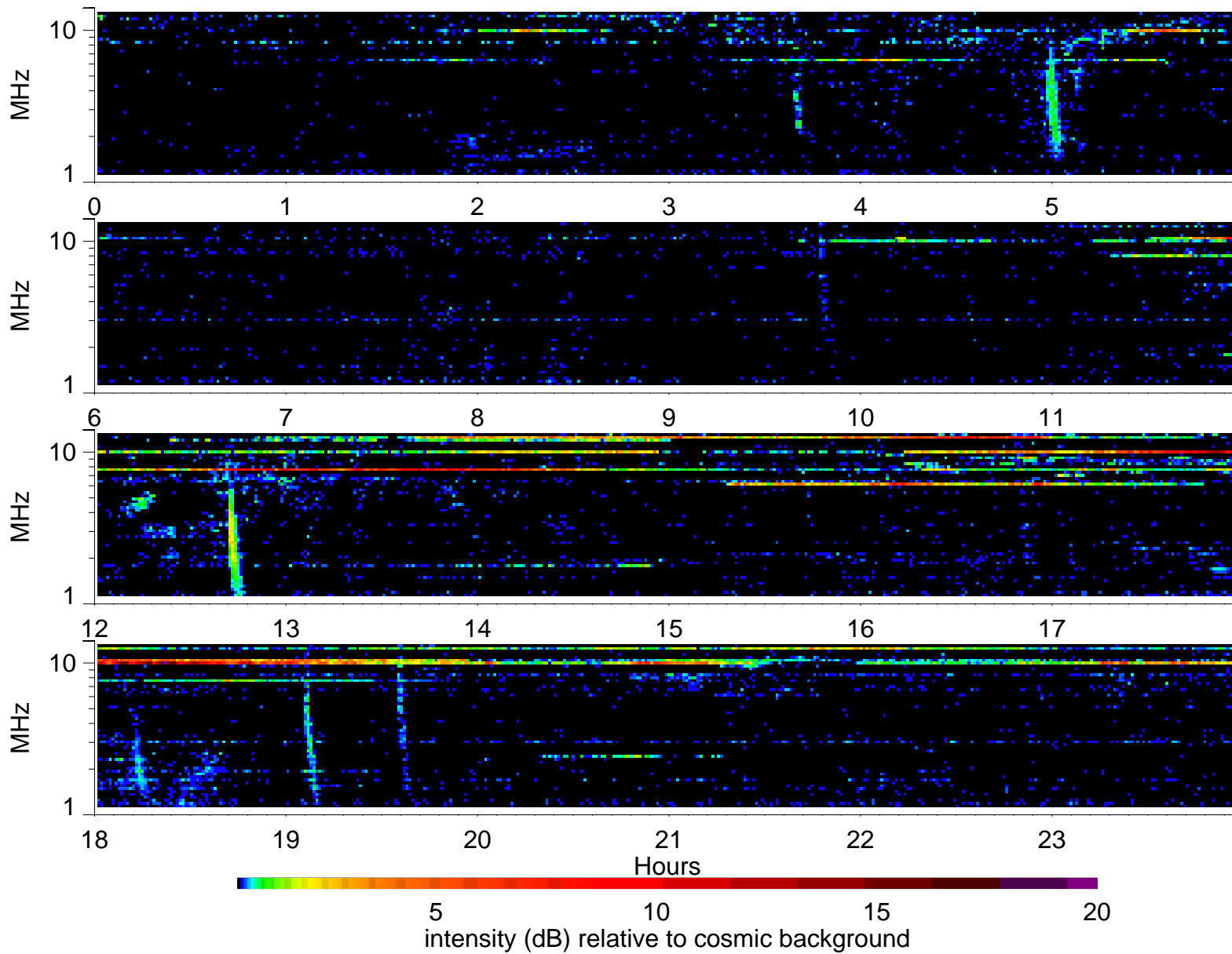
Wind Waves RAD2 receiver: 2000/12/12
