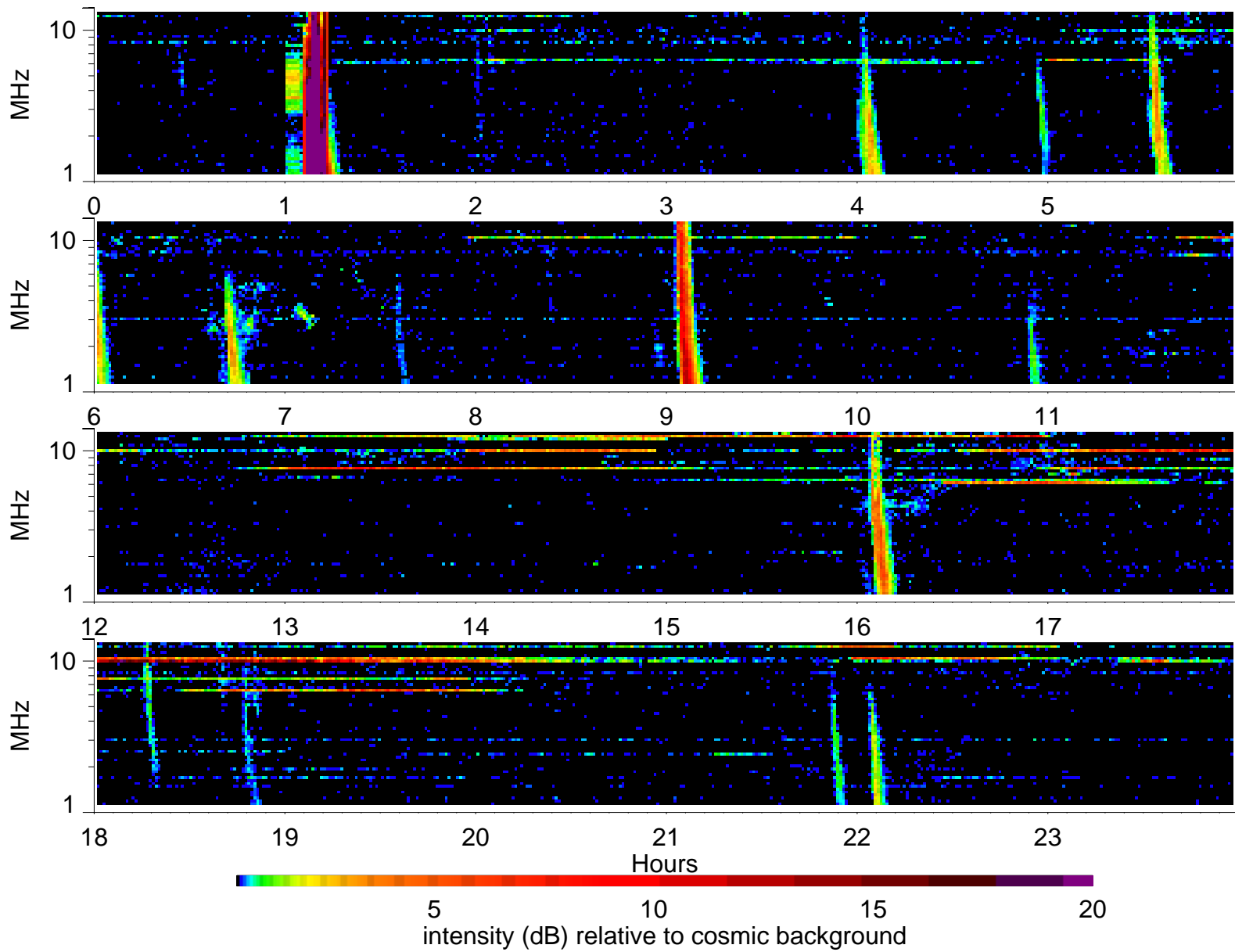
Wind Waves RAD2 receiver: 2000/12/11
