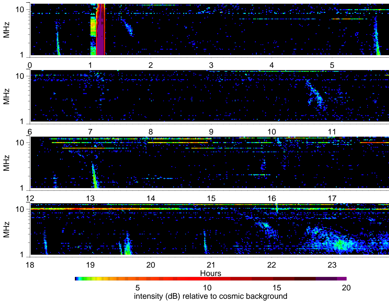
Wind Waves RAD2 receiver: 2000/12/9
