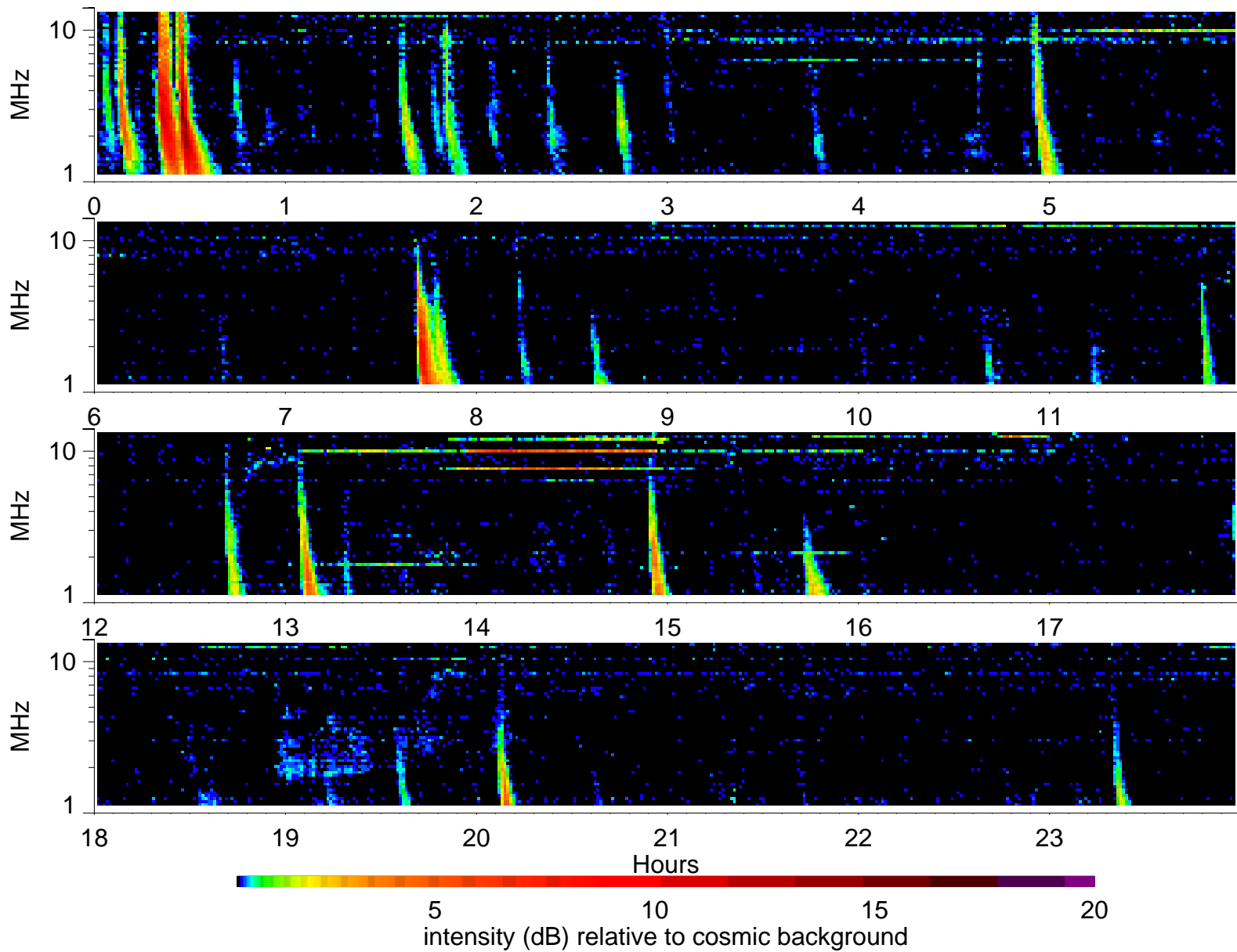
Wind Waves RAD2 receiver: 2000/12/8
