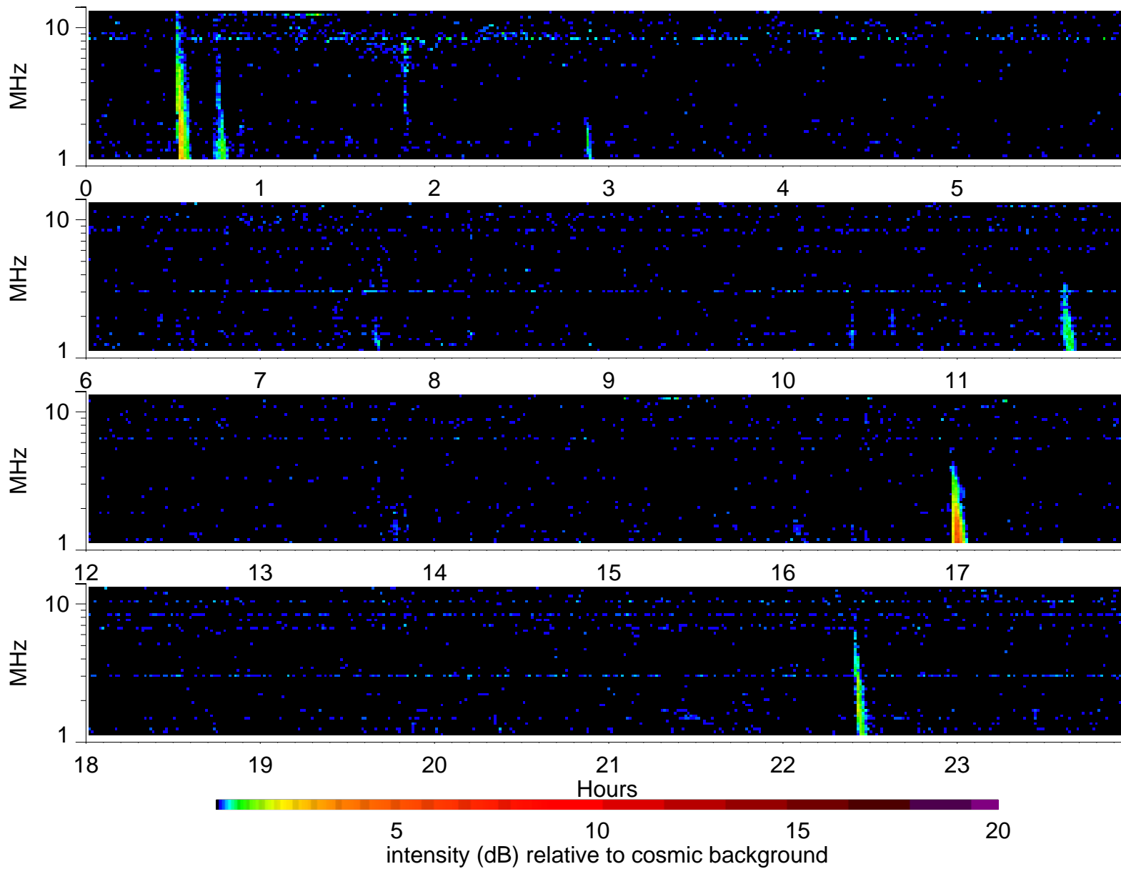
Wind Waves RAD2 receiver: 2000/12/4
