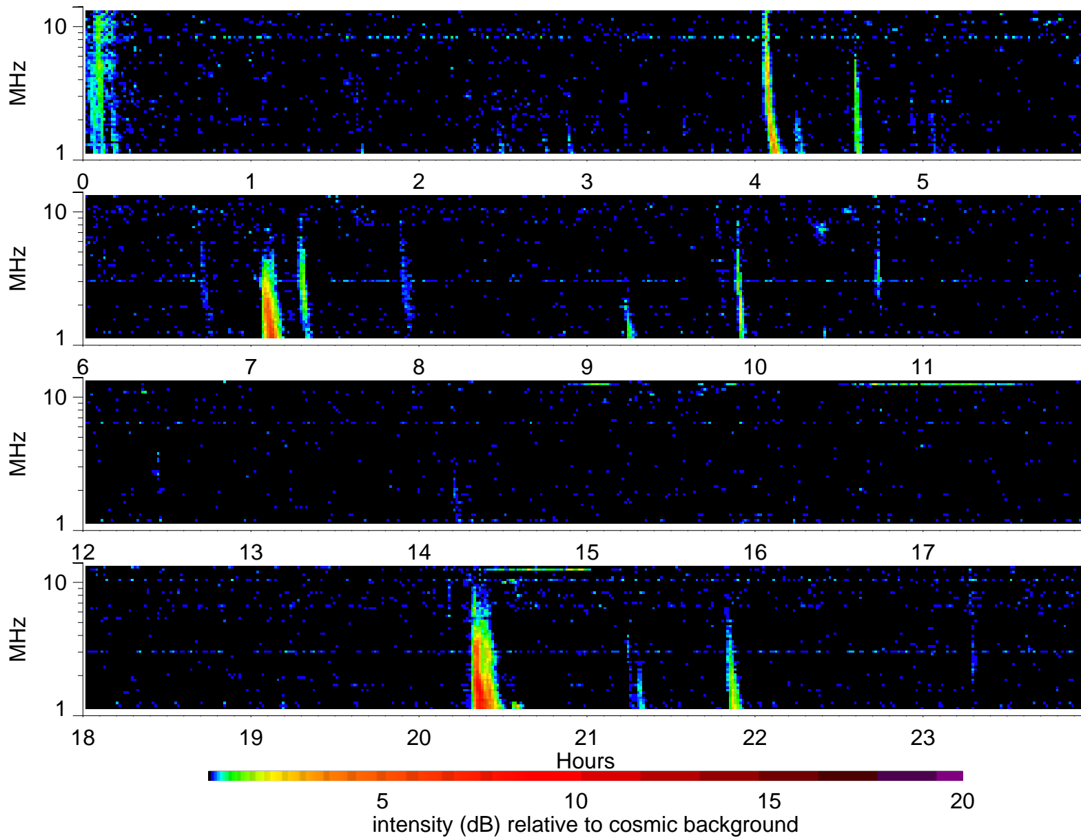
Wind Waves RAD2 receiver: 2000/12/2
