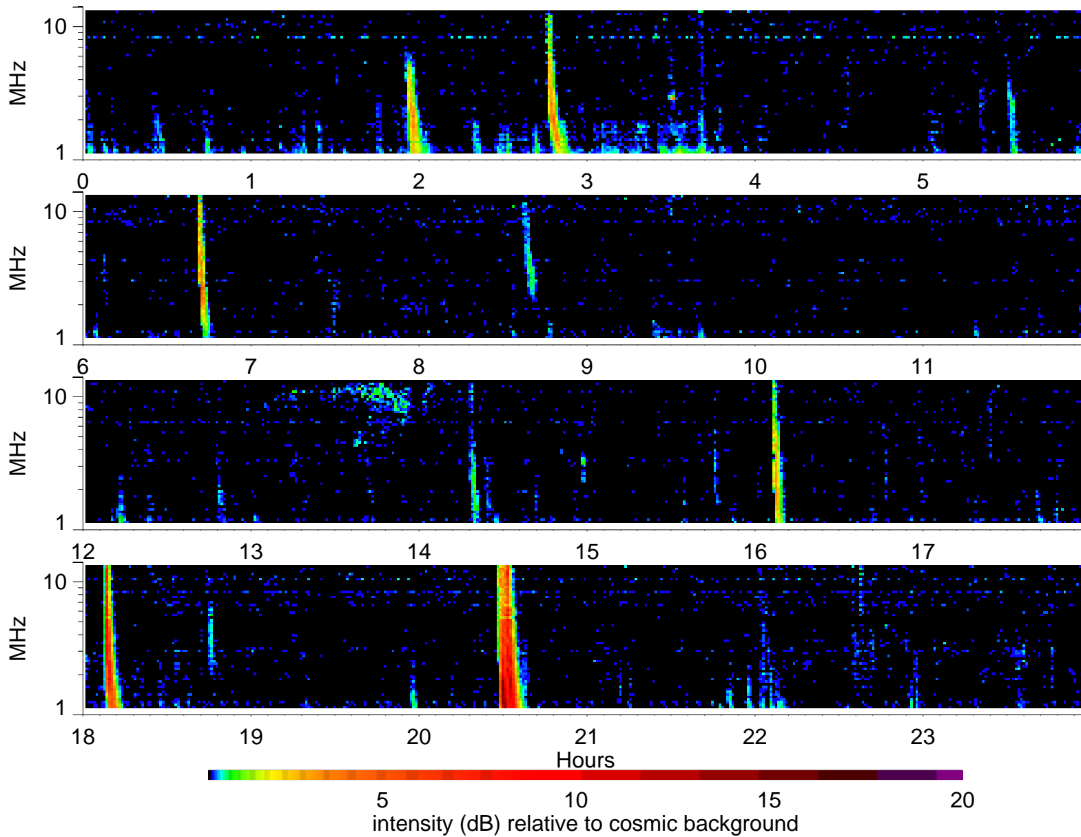
Wind Waves RAD2 receiver: 2000/11/30
