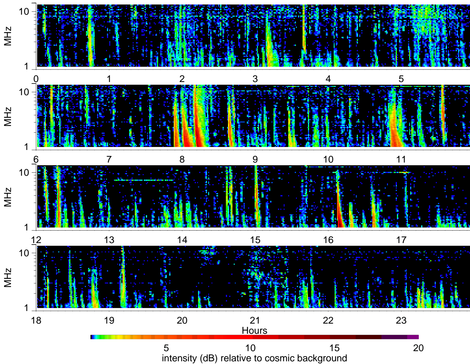
Wind Waves RAD2 receiver: 2000/11/28
