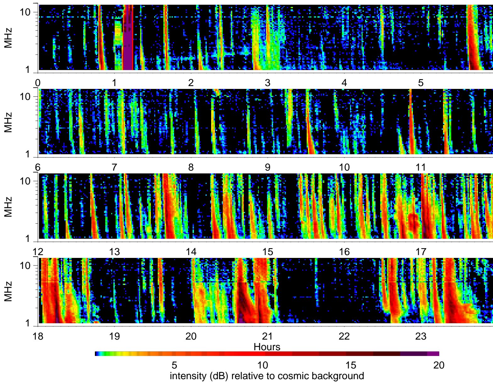
Wind Waves RAD2 receiver: 2000/11/23
