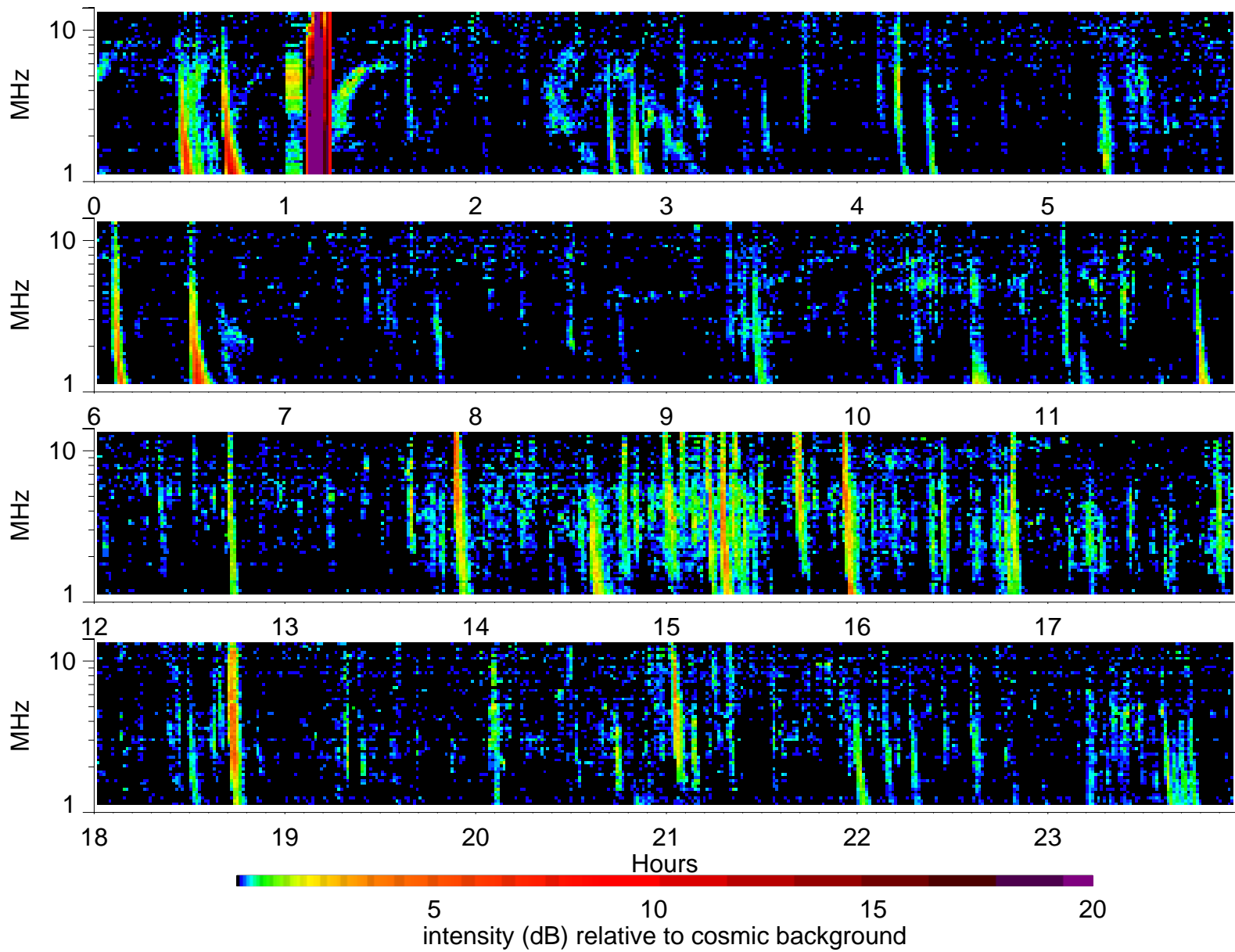
Wind Waves RAD2 receiver: 2000/11/21
